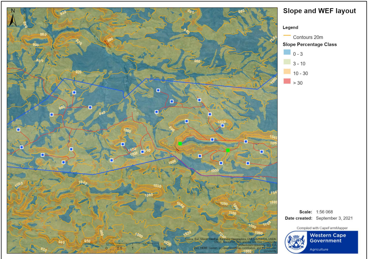
Figure 20: Koup 1 slope classification (%) excerpt (Figure 18) showing proposed WEF development infrastructure. The proposed turbines indicated in green are currently located on slopes over 10%. Some of the proposed access road infrastructure on the eastern portion of the site is located on slopes over 10%.
