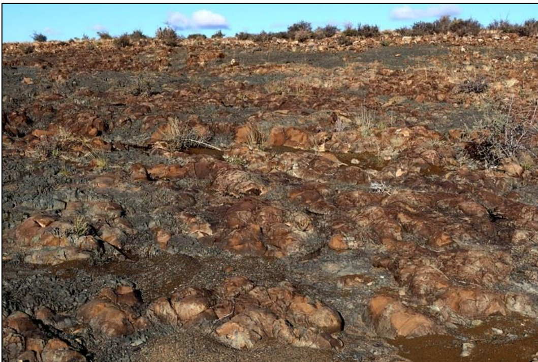
Figure 12: Horizon of large (boulder-sized), spheroidal concretions of rusty-brown ferruginous carbonate within the Karelskraal Member in the Koup 2 WEF project area (Farm 1/380).
