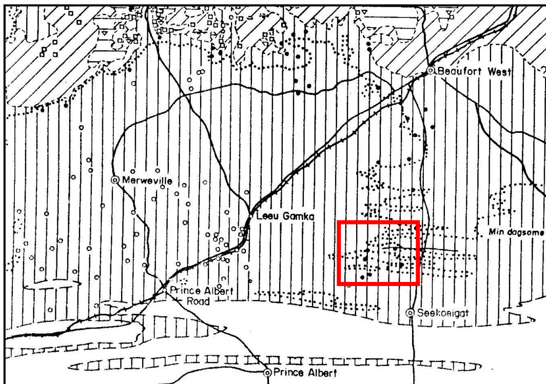
Figure 21: Vertebrate fossil localities within the Lower Beaufort Group in the region south of Beaufort West where the boundary between the Abrahamskraal and Teekloof Formations is highly folded
