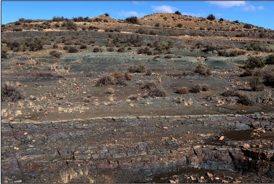
Figure 11: Outstanding exposures of multi-hued Karelskraal Member mudrocks with intercalated thin, pale crevasse splay sandstones capped by Poortjie Member sandstones, Koup 2 WEF project area (Farm 1/380).
