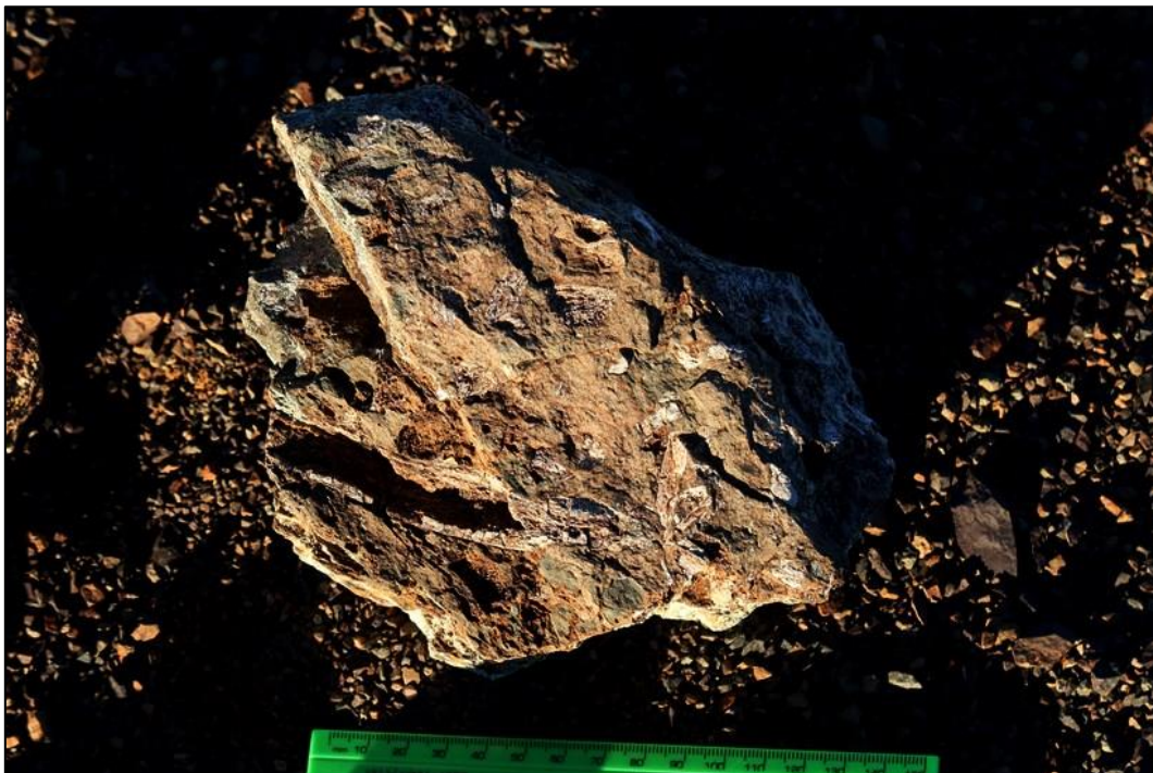
Figure 37: Close up of one of the sandstone and bone blocks illustrated above showing highly fragmentary preservation, possibly due to sun-cracking during pre-burial exposure on the ancient Karoo floodplain (Loc. 660) (Scale in cm).
