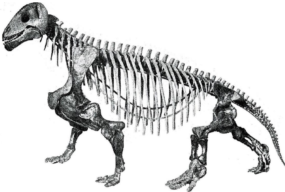
Figure 24: Skeleton of the tapinocephalid (thick-skulled) dinocephalian Moschops , a rhino-sized herbivorous therapsid that reached lengths of 2.5 to 3 m and may have lived in small herds. Postcranial remains (and much rarer fossil skull material) of several dinocephalians have been recorded within and just outside the Koup WEF project area.
