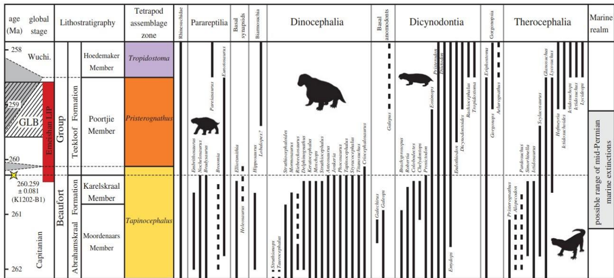
Figure 22: Chart showing the ranges of known terrestrial tetrapod genera from the Middle to Late Permian of the Main Karoo Basin (From Day et al. 2015b). The boundary between the Abrahamskraal and Teekloof Formations is associated with a catastrophic extinction event at the end of the Capitanian Stage (c. 260 Ma) that has been dated here on the basis of a tuff horizon close to the contact of the Karelskraal and Poortjie Members (yellow star). Key victims of the extinction event were almost all the large-bodied dinocephalians and pareiasaur parareptiles as well as many (but not all) dicynodonts and therocephalians.
