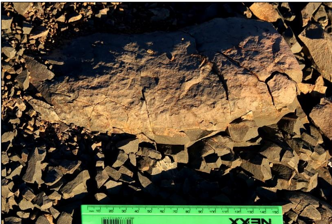
Figure 55: Convex sandstone cast of a small vertebrate burrow weathering out of cleaved Poortjie Member mudrocks (Loc. 688) (Scale in cm and mm).
