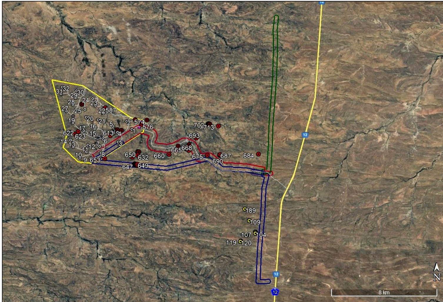
Figure 59B: Google Earth© satellite image showing new (red) and previously recorded (yellow) fossil sites within the Lower Beaufort Group in the context of the Koup 2 WEF and grid connection project areas (Please see following satellite map for more detail).
