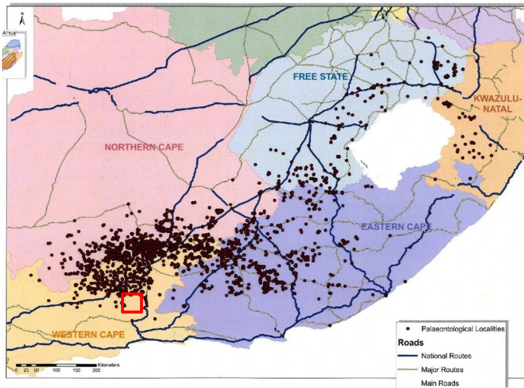
Figure 20: Distribution of recorded vertebrate fossil sites within the southern portion of the Main Karoo Basin (modified from Nicolas 2007). The approximate location of the combined Koup WEF project area to the south of Beaufort West (BW) is indicated by the red rectangle. The high density of recorded fossil sites along the N12 here as well as further to the north is notable.
