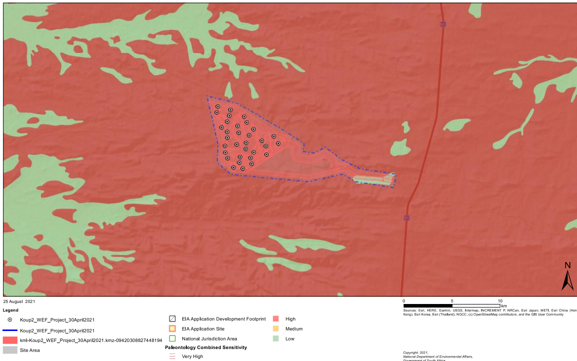
Figure 58: Paleontological sensitivity map for the Koup 2 WEF and grid connection project area. Due to the scarcity of well-preserved, scientifically important fossils over much of this region, based on desktop studies and fieldwork, it is inferred that large parts of the project area are in practice of LOW palaeontologically sensitivity. However, there is also a substantial number of, dispersed and unpredictable fossil sites here of HIGH to VERY HIGH sensitivity. Applying the precautionary principle, the Koup 2 WEF and associated grid connection project area are best assigned an overall High Sensitivity as far as palaeontological heritage is concerned. Areas underlain by thick alluvial sediments are generally of LOW sensitivity, although important concentrations of Cenozoic mammal remains might occur here.
