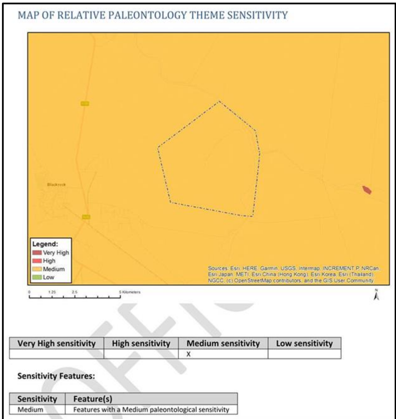
Figure 6: DFFE Screening tool palaeosensitivity map also shows the areas as having medium sensitivity. (Note that colour coding by SAHRIS and the DFFE differ but the sensitivity level is the same – medium/moderate).
