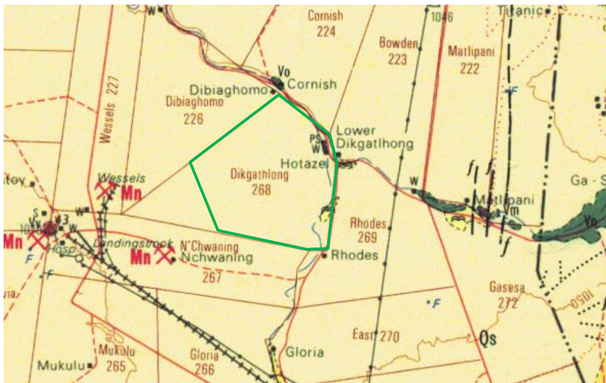
Figure 4: Geological map of the area around the Farm Dikgathlong 268. The location of the proposed project is indicated within the green polygon. Abbreviations of the rock types are explained in Table 2. Map enlarged from the Geological Survey 1: 250 000 map 2722 Kuruman.
