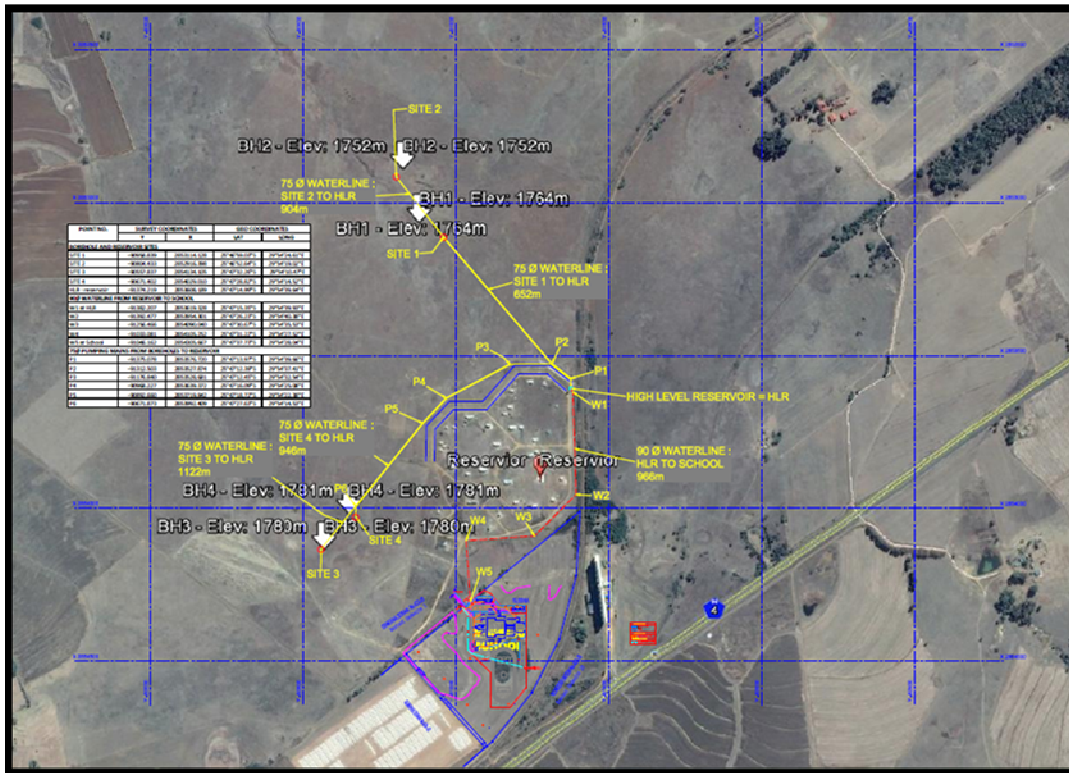
Figure 1: Proposed Layout plan (AdiEnvironmental).
