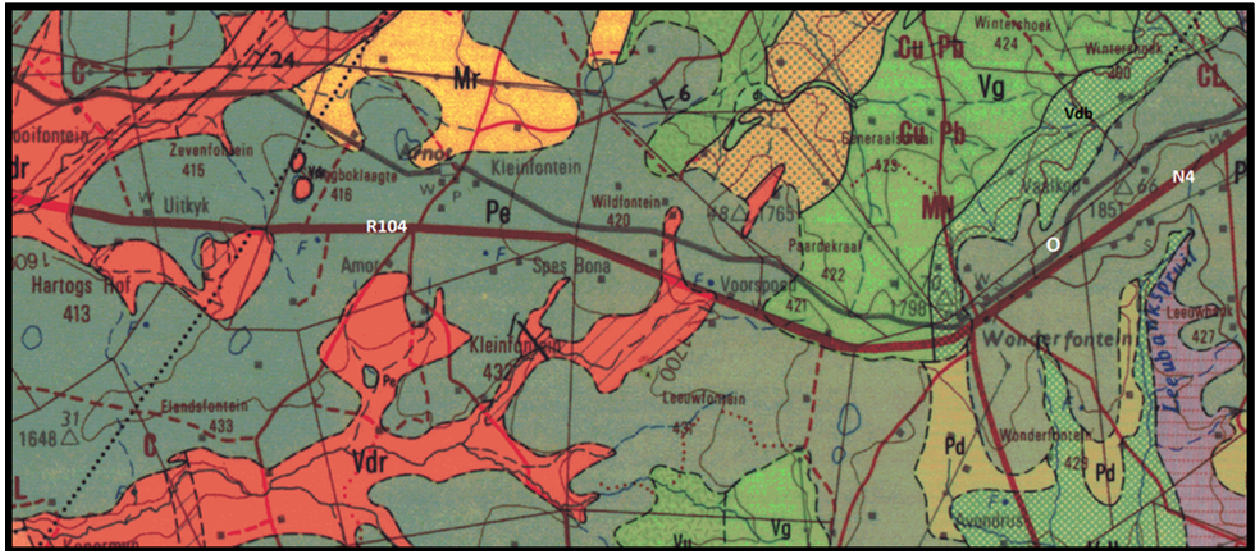
Figure 5: The geology of the development area.
