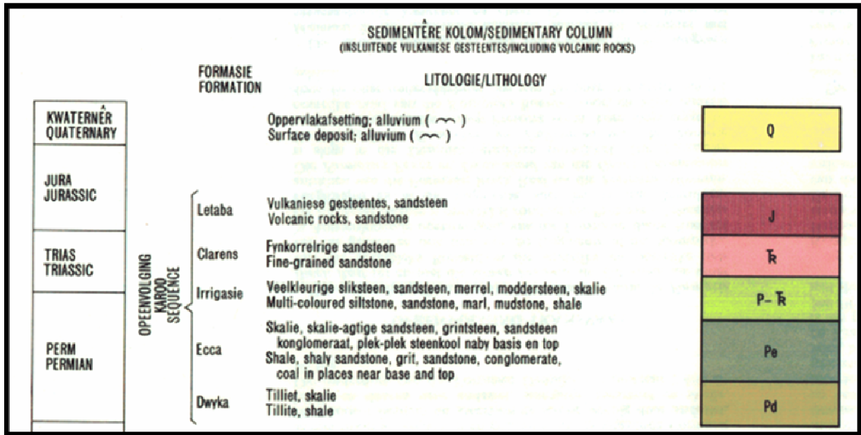
Figure 6: Lithostratigraphic column to show the Ecce Group (Walraven 1978).
