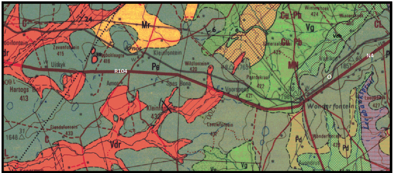
Figure 5: Excerpt of 1:250 000 Geological Map 2528 Pretoria (Walraven 1978).
