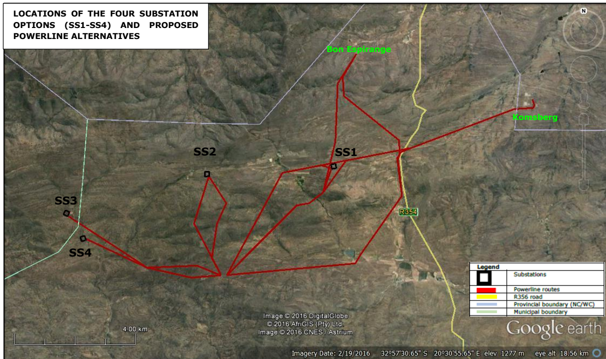
Figure 4: View of the locations of the four substation positions (SS1 – SS4) proposed within the Brandvalley WEF area
