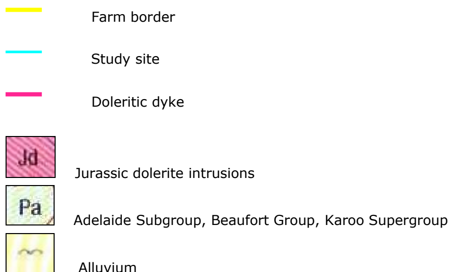
Figure 2: Geological Map of the study area and surroundings (adapted from the 3124 MIDDELBURG 1: 250 000 Geology Map, Geological Survey, 1996)
