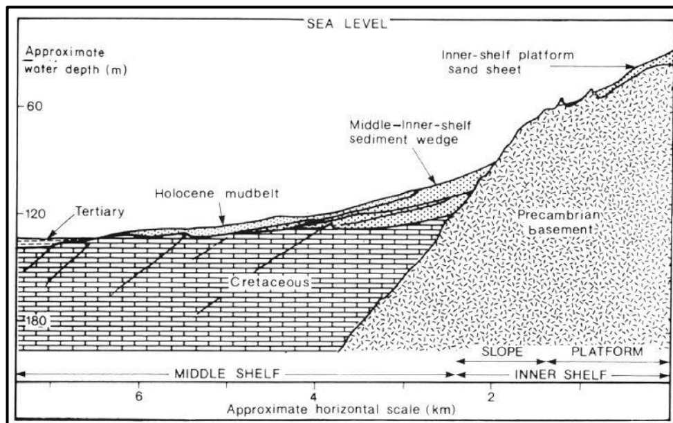
Figure 3. Schematic geology of the shallow continental shelf based on geophysical seismic profiles, illustrating the “mudbelt” sediment wedge overlying the inner to midshelf transition. Adapted from Birch et al., 1991.
