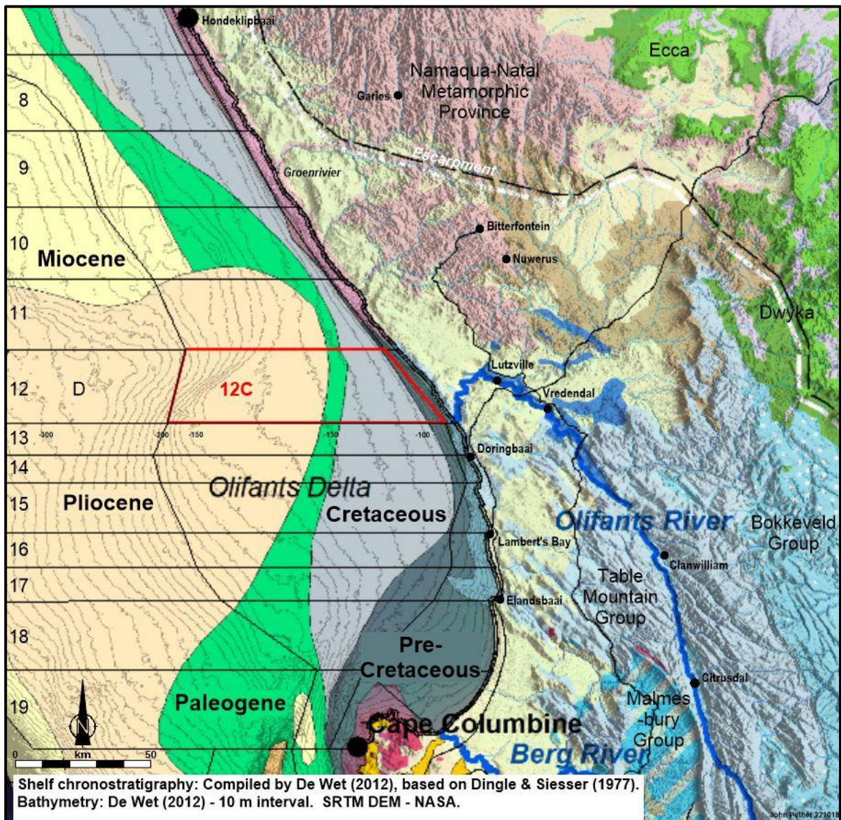
Figure 1. Location of Sea Concession 12C and regional geological context.
