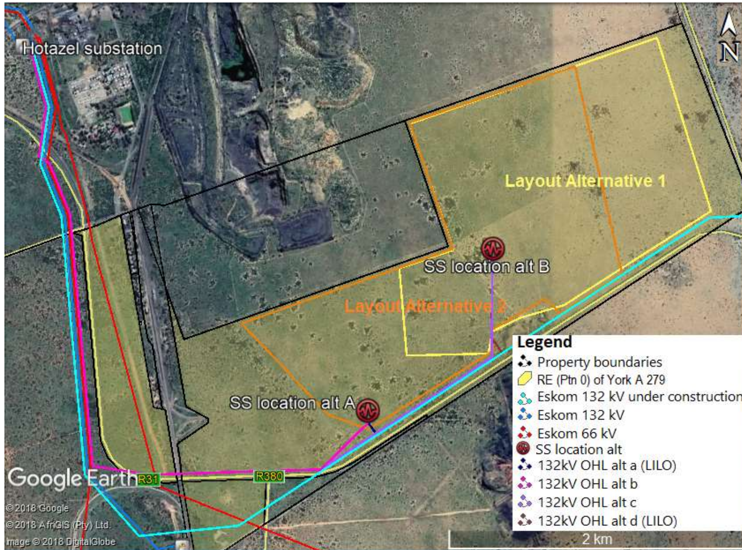
Figure 1: Google Earth© satellite image of the Hotazel Solar PV facility project area on York A, Farm No. 279 Portion 0 near Hotazel, Northern Cape (Option 1 = yellow polygon. Option 2 = orange polygon). Various 132 kV overhead transmission line route options to Hotazel Substation are indicated in lilac, blue, pink and maroon. Onsite substation alternative sites A & B are shown by red symbols.
