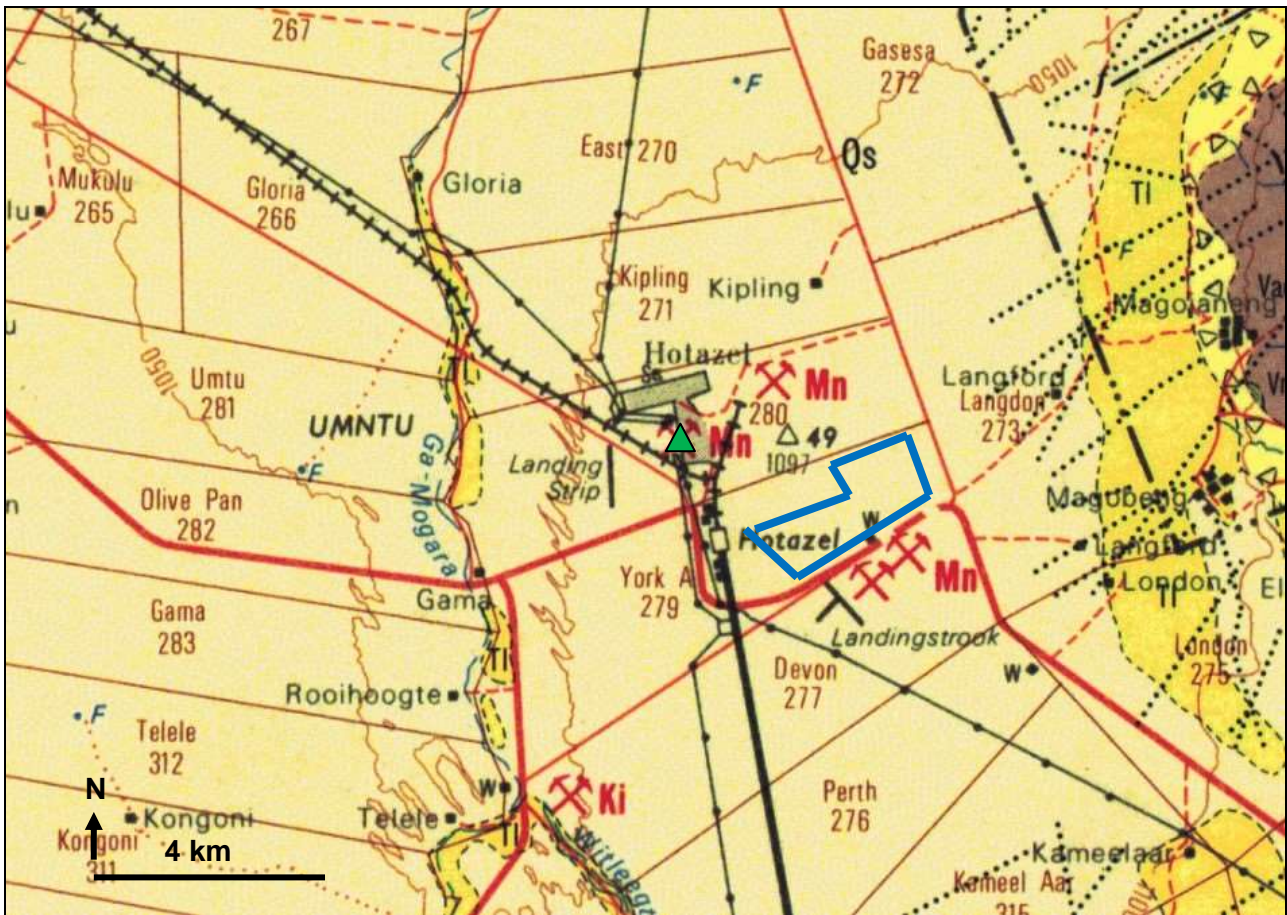
Figure 2: Extract from 1: 250 000 geology map 2722 Kuruman (Council for Geoscience, Pretoria) showing location of the York A, Farm No. 279 Portion 0 project area for the proposed Hotazel Solar PV Facility (blue polygon) to the SE of Hotazel, Northern Cape. The green triangle is the existing Hotazel Substation. The entire project area, including the proposed 132 kV overhead transmission line route options to Hotazel Substation, is underlain by aeolian sands of the Gordonia Formation (Kalahari Group) (Qs, pale yellow areas on the map). These are extensively underlain by thick near-surface calcrete that crop out at surface along the Ga-Mogara River to the west and around pans (TI, darker yellow).
