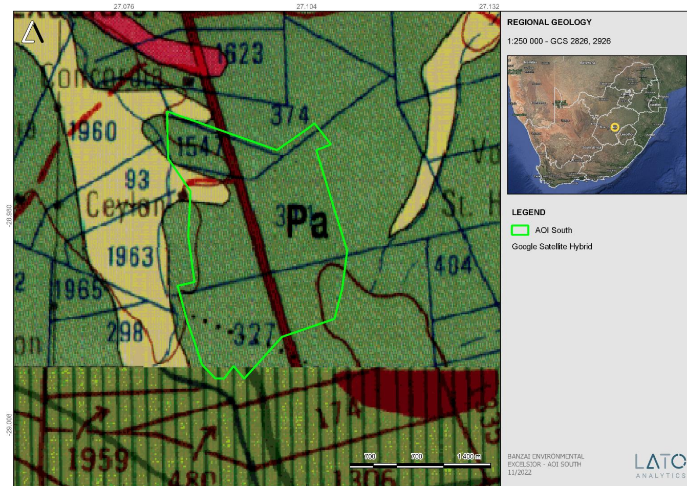
Figure 3: Extract of the 1:250 000 Winburg 2826 (1987) and the Bloemfontein 2926 (1966) Geological Map (Council for Geosciences, Pretoria) indicating the proposed Lengana SPP development near Excelsior in the Free State.
