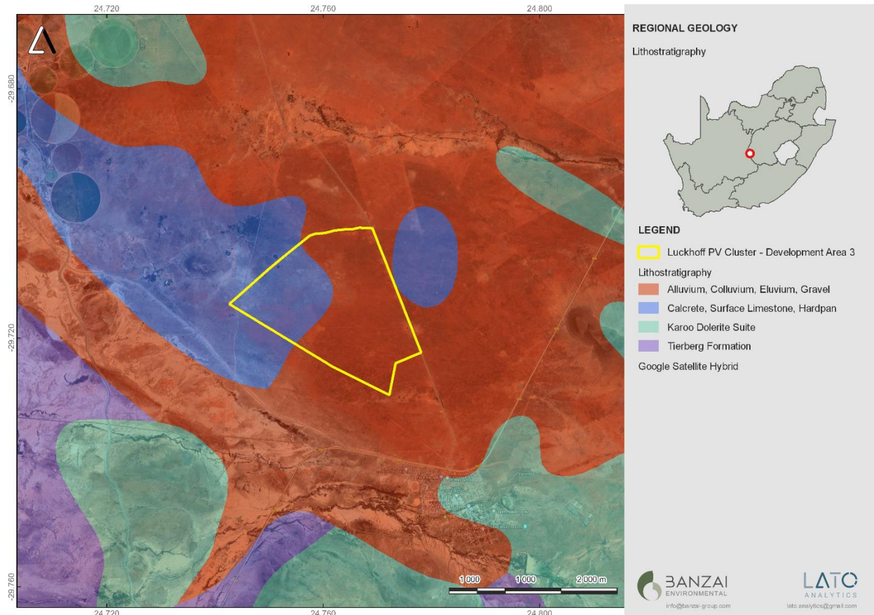
Figure 6: Updated Geology (Council of Geosciences, Pretoria) indicates that the proposed Luckhoff Solar 3 Solar Energy Facility in the Free State Province is underlain by underlain by calcrete, surface limestones and Hardpan as well as alluvium, colluvium, eluvium, gravel, scree, sand, soil and debris.
