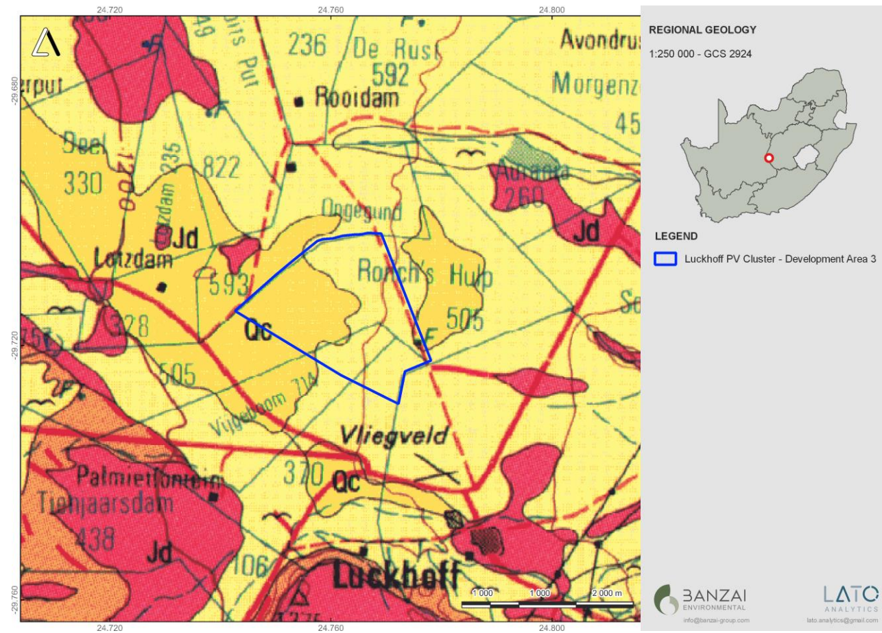
Figure 4: Extract of the 1:250 000 Koffiefontein 2924 Geological map (1992) (Council of Geoscience, Pretoria) indicating the geology of the Luckhoff Solar 3 Solar Energy Facility in the Free State Province. The development is underlain by Caenozoic aeolian sand (Qs) as well as calcrete (Qc, yellow).
