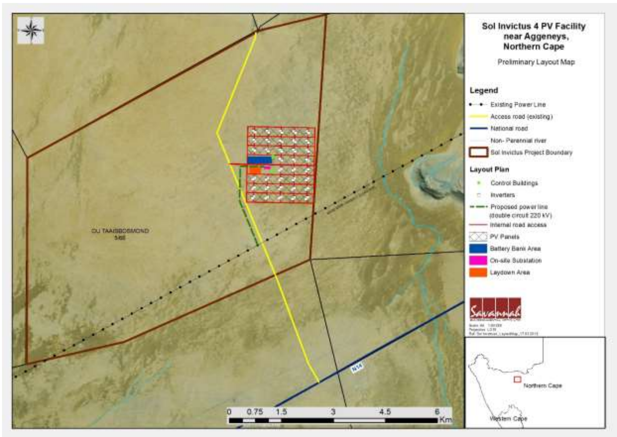
Figure 2: Aerial view of the study area showing the Portion 5 of farm 66 (brown polygon), the proposed Sol Invictus 4 PV facility (red square), the proposed transmission line (green dashed line) and the existing access road (yellow line) leading north from the N14 (blue line).
