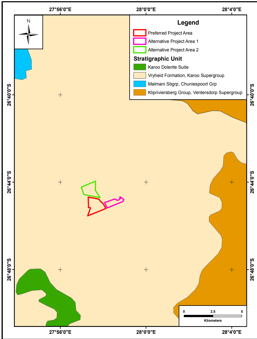
Figure 2: Geological map of the area underlying the preferred and both alternative project areas as well as within their immediate environs.
