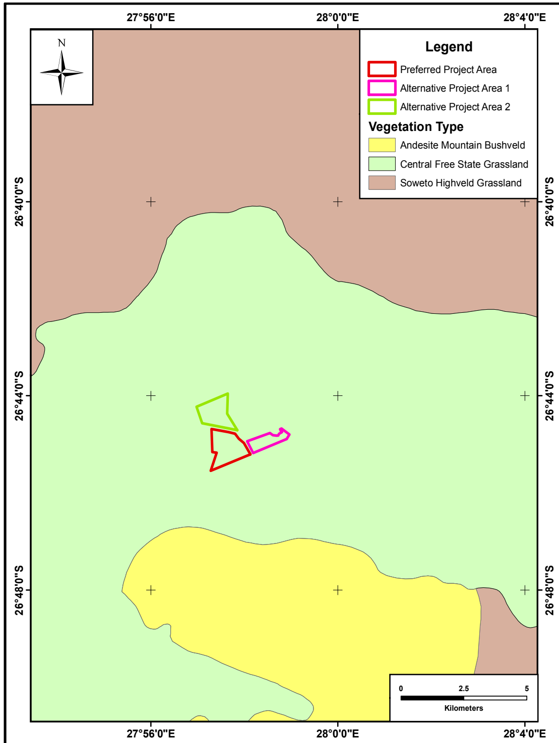
Figure 6: Map of the distribution of the vegetation veld types located beneath the three potential project areas and within their immediate environs (after Mucina and Rutherford, 2006).
