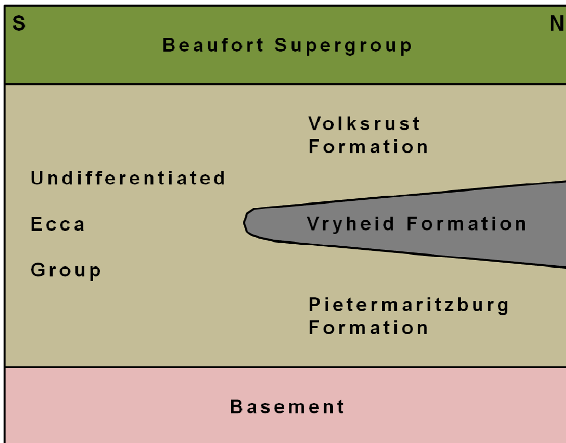
Figure 3: Schematic north-south oriented stratigraphic section of the Ecca Group in the north-east corner of the Karoo Basin. The Volkswrust and Pietermaritzburg Formations can only be recognised when the Vryheid Formation forms part of the vertical sequence. In the north and north-western portions of the basin the Pietermaritzburg Formation was not deposited and the coal-bearing strata of the Vryheid Formation rest directly upon the basement.
