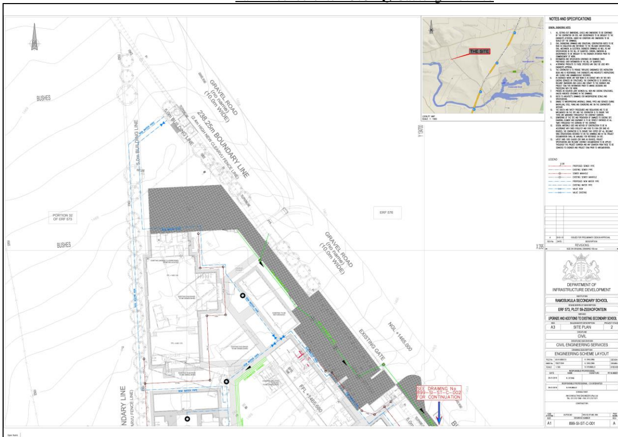
Figure 8: Proposed layout of the proposed re-modelling and expansion of the school
