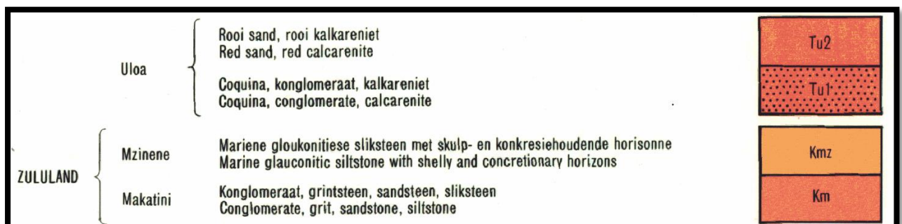
Figure 3: Lithostratigraphic column of the development area (Kosi Bay).
