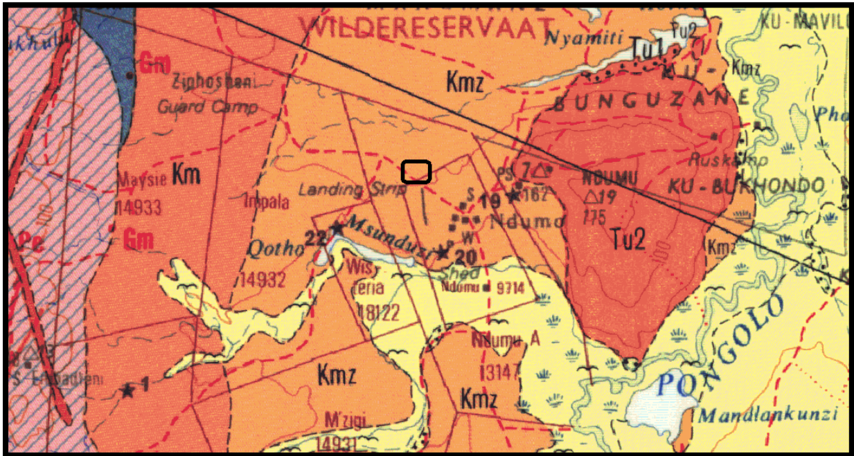
Figure 2: Geology of the development area (1h).
