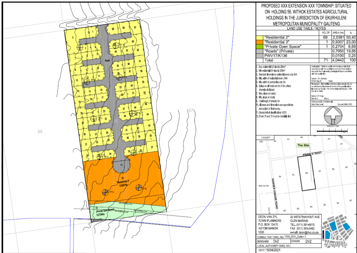
Figure 1: Lay-out plan of development (I. Tshabalala).
