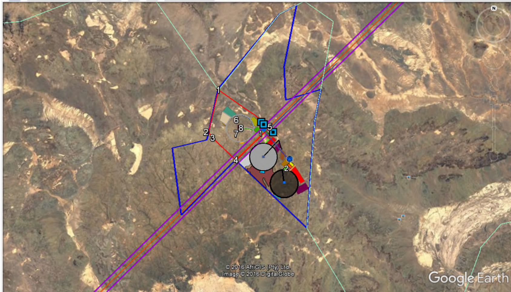
Fig. 2. Revised layout for the proposed SolarReserve Kotulo Tsatsi CSP 1, 2 & 3 and PV Solar Energy Facilities near Kenhardt.
