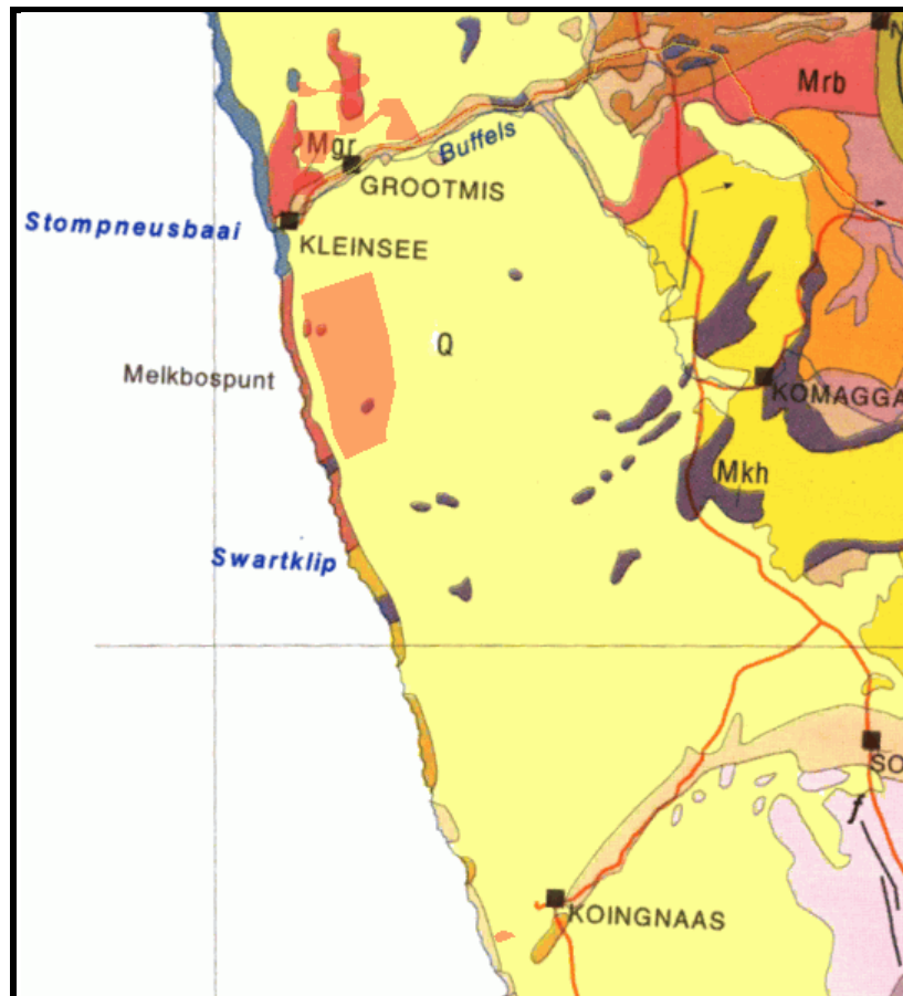
Figure 2. Project areas located on 1:1000000 Geological Map (CGS, 1997).
