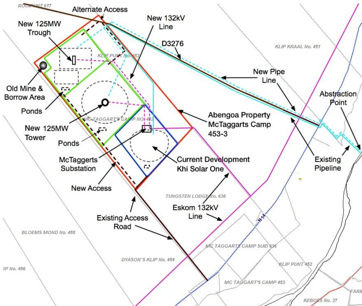
Map indicating the proposed Upington Solar Thermal Plant Two (and other phases) and associated infrastructure on Portion 3 of the Farm McTaggart's Camp.
