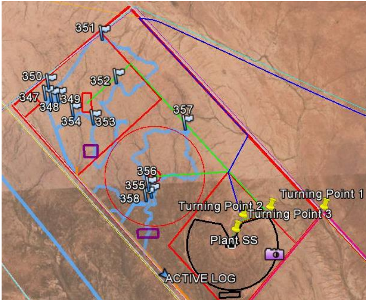
Footprint areas of the Upington Solar Thermal Plant Two north-west of the current Khi Solar 1 development, showing GPS tracks.
