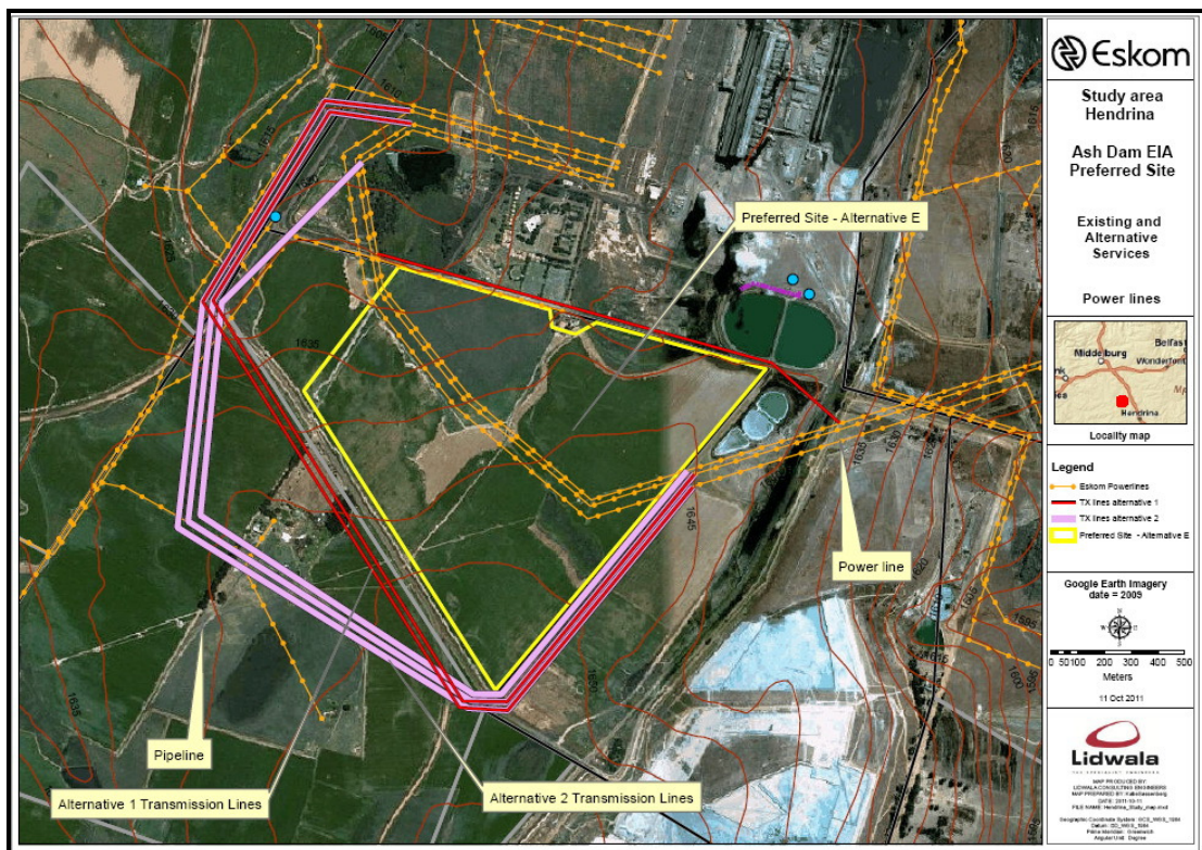
Fig. 4. Map showing the rerouting alternatives for the power lines.
