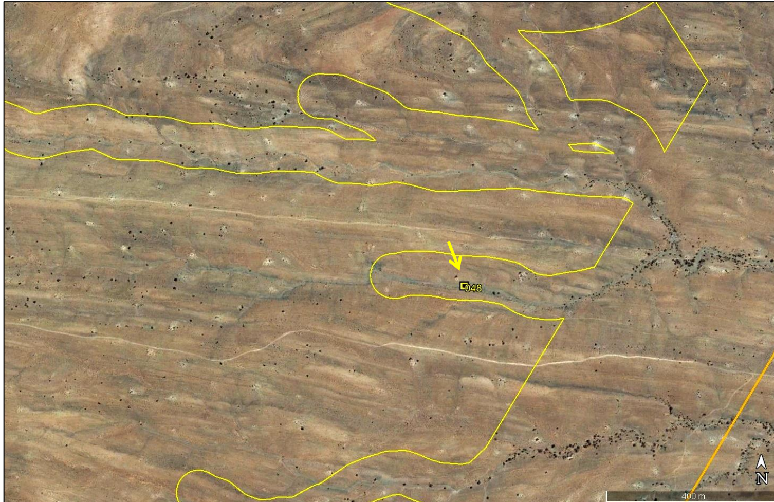
Figure A1.2. Satellite map showing new fossil sites within the south-eastern sector of the Heuweltjies WEF project area (yellow polygon). The pareiasaur reptile skeleton in a stream bank at Loc. 048 (arrow) lies outside the proposed WEF buildable area (yellow polygons) and will be protected within the ecological buffer zone along drainage lines.
