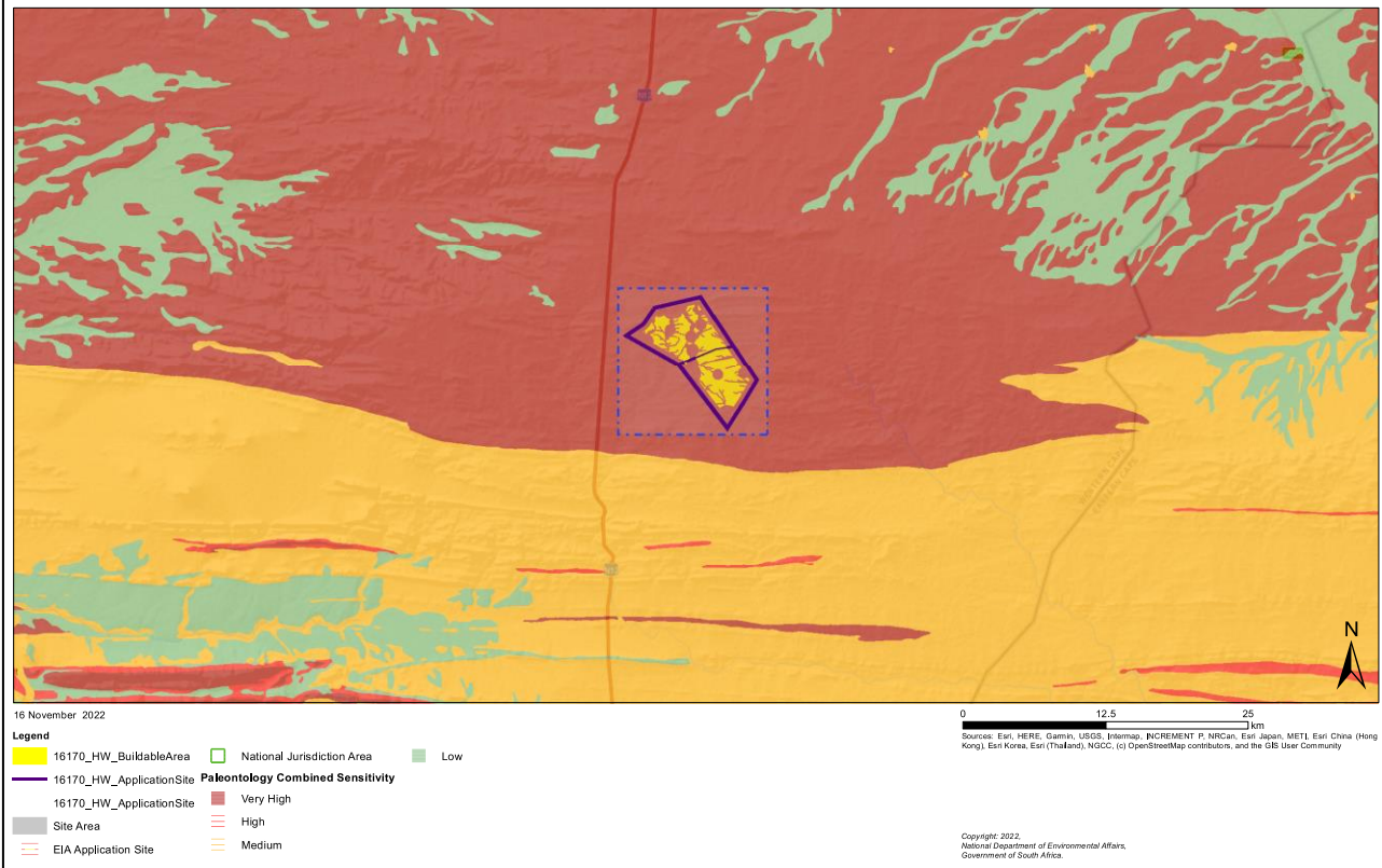
Figure 48: Provisional paleontological sensitivity map for the Heuweltjies WEF project area based on the DFFE Screening Tool indicating that the entire project area is of Very High Palaeosensitivity. Due to the scarcity of well-preserved, scientifically important fossils over much of this region, based on desktop studies and fieldwork, it is inferred that most parts of the project areas are in practice of LOW palaeontologically sensitivity. Areas underlain by thick alluvial sediments here are generally of LOW sensitivity, although important concentrations of Caenozoic mammal remains might occur here. The palaeosensitivity mapping shown by the DFFE Screening Tool is contested here.
