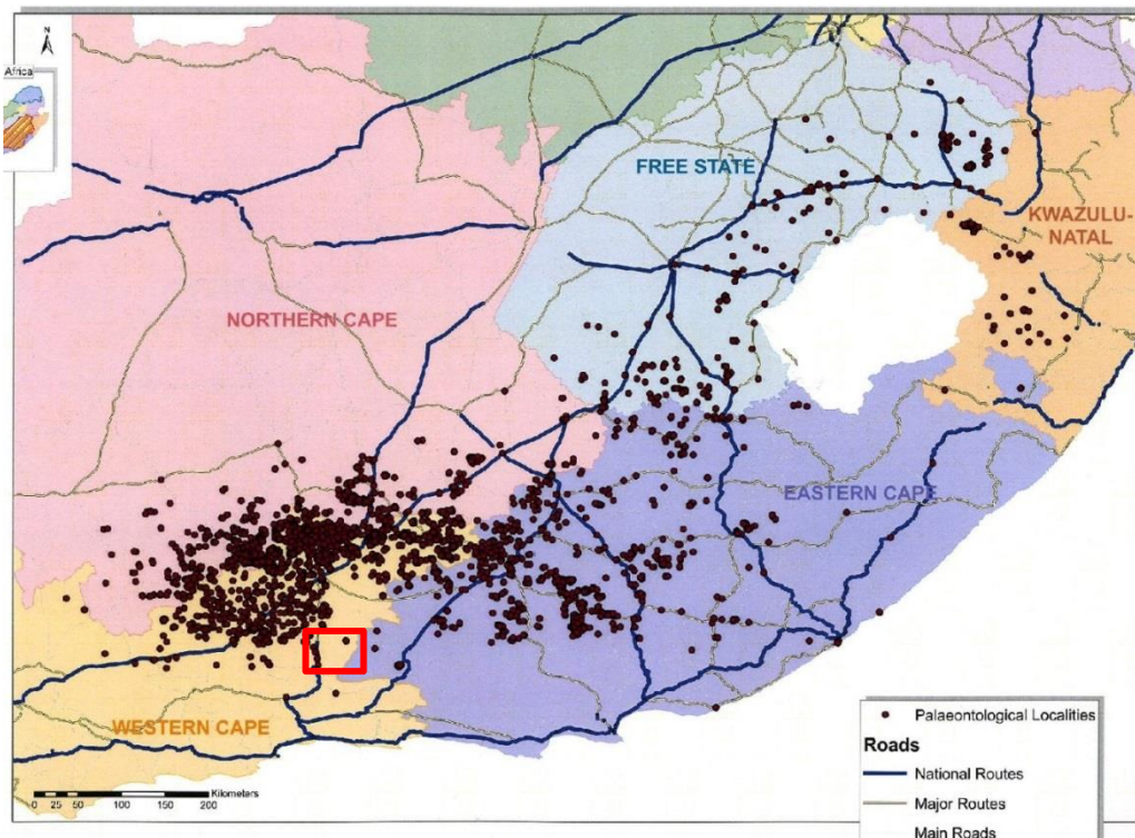
Figure 39: Distribution of recorded vertebrate fossil sites within the within the Lower Beaufort Group of the Main Karoo Basin (modified from Nicolas 2007). The WEF project area to the south of Beaufort West is located within the small red rectangle. The very low density of recorded fossil sites here, to the east of the N12 and on the SW periphery of the Aberdeen Vlaaktes , is notable.
