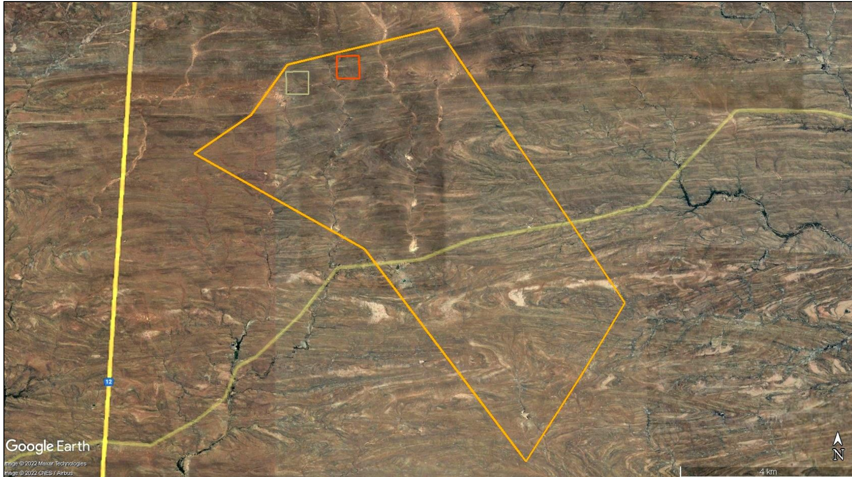
Figure 34: Google Earth© satellite image showing the Heuweltjies WEF project area (orange polygon) and on-site substation options (grey and orange squares). The pronounced east-west grain of the Palaeozoic bedrocks, a consequence of pronounced Permo-Triassic folding and faulting during the Cape Orogeny, is clearly seen here. Paler areas reflect (1) cover by surface gravels such as vein quartz and tuffite or (2) Late Caenozoic alluvium along major drainage lines.
