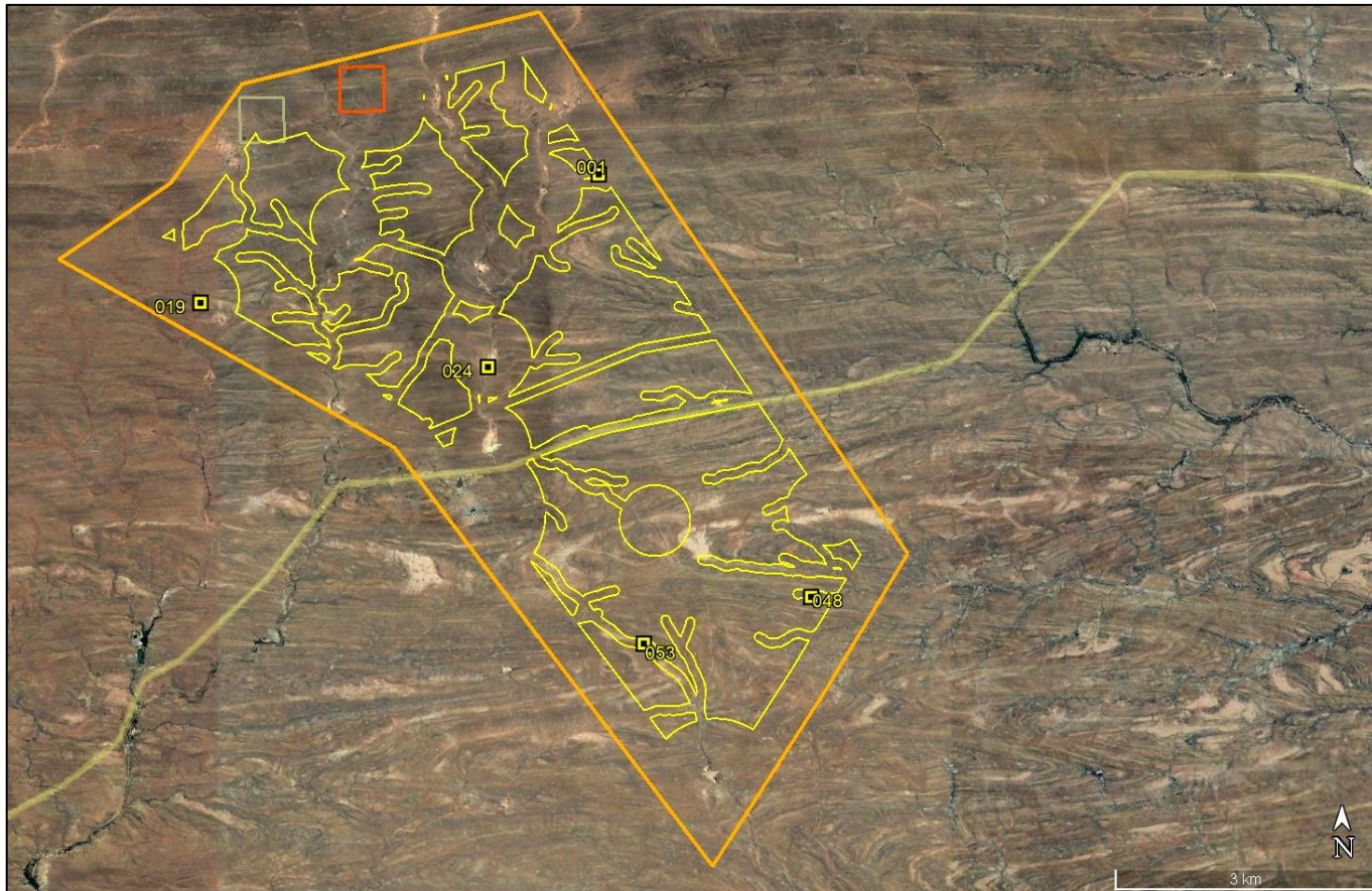
Figure A1.1: Google Earth© satellite image of the Heuveltjies WEF and associated Infrastructure project area (orange polygon) showing numbered fossil sites recorded here (numbered yellow squares). See table above for GPS data and brief description for the new Heuveltjies WEF fossil sites. Many of the recorded fossil sites are protected within standard environmental buffer zones along drainage lines and none of them lie within the proposed buildable area (yellow polygons). No palaeontological heritage High Sensitivity or No-Go areas have been defined within the WEF project area since well-preserved, scientifically important fossils are very sparse here and, in all cases, known or chance fossil finds can normally be effectively mitigated through professional recording and collection during the pre-construction phase, if necessary.
