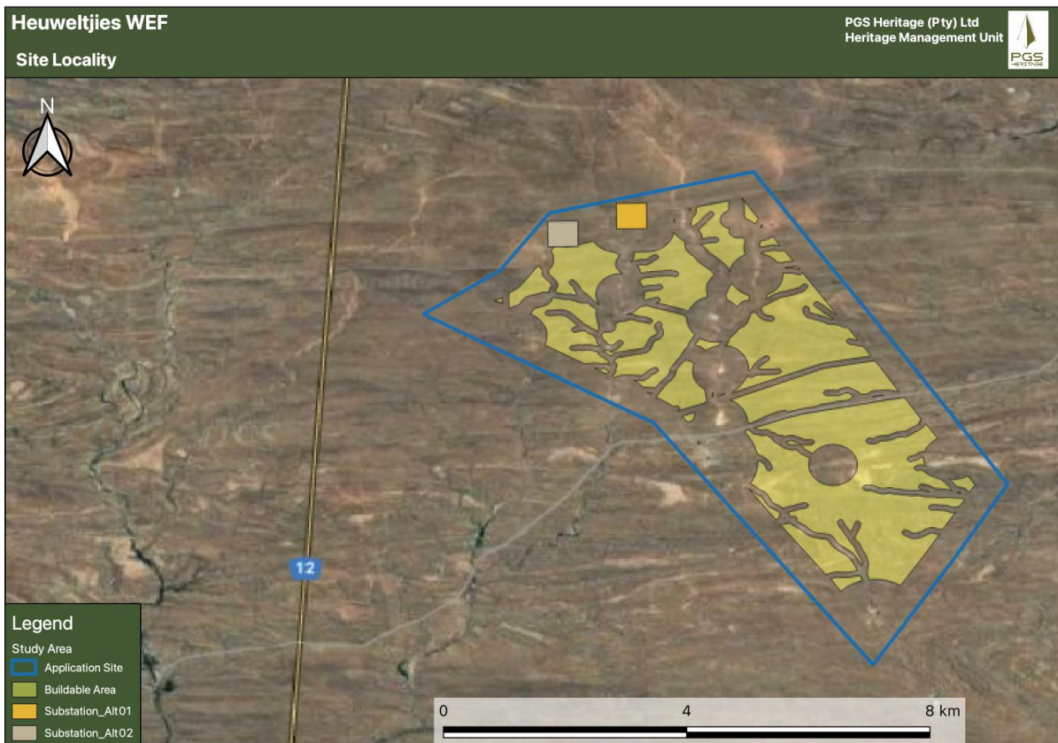
Figure 3: Preliminary layout for the Heuweltjies WEF.
