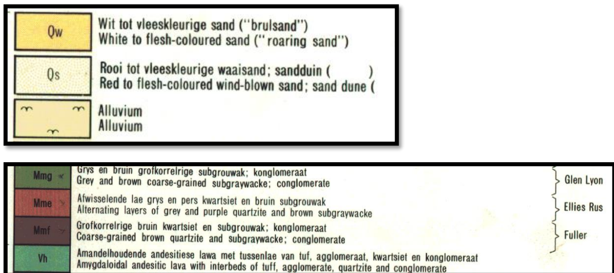
Figure 4: Lithology (Moen 1977).
