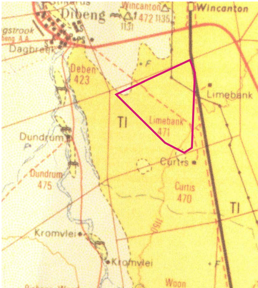
Figure 3. Geological map of the study area (portion of 1:250 000 scale geological map (2722 Kuruman)).
