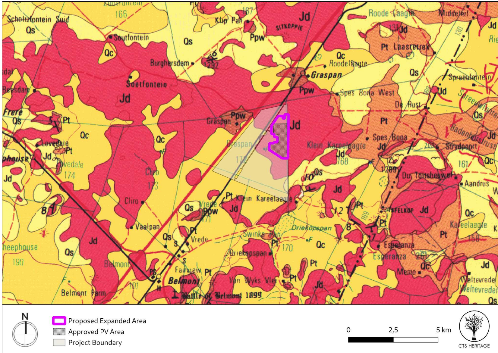
Figure 4b. Geology Map. Extract from the CGS 2924 Koffiefontein Map indicating that the development area for the Graspan PV is underlain by Quaternary Sands (Qc) and Jurassic Dolerite (Jd)
