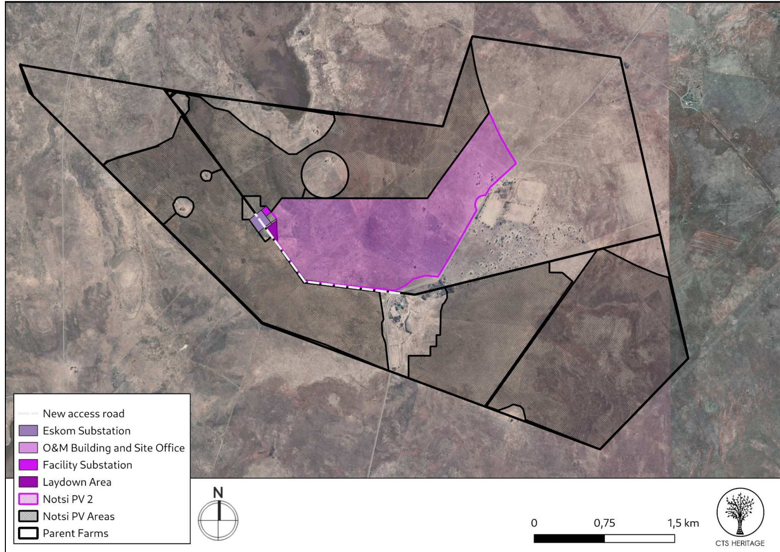
Figure 1.2: The proposed development layout of Notsi PV 2 Facility
