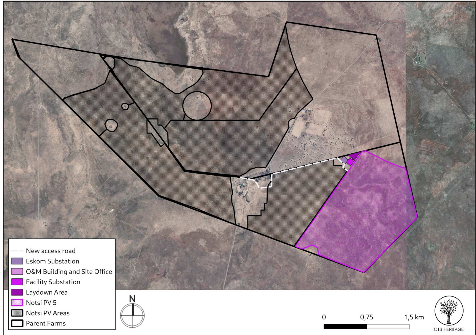
Figure 1.2: The proposed development layout of Notsi PV 5 Facility
