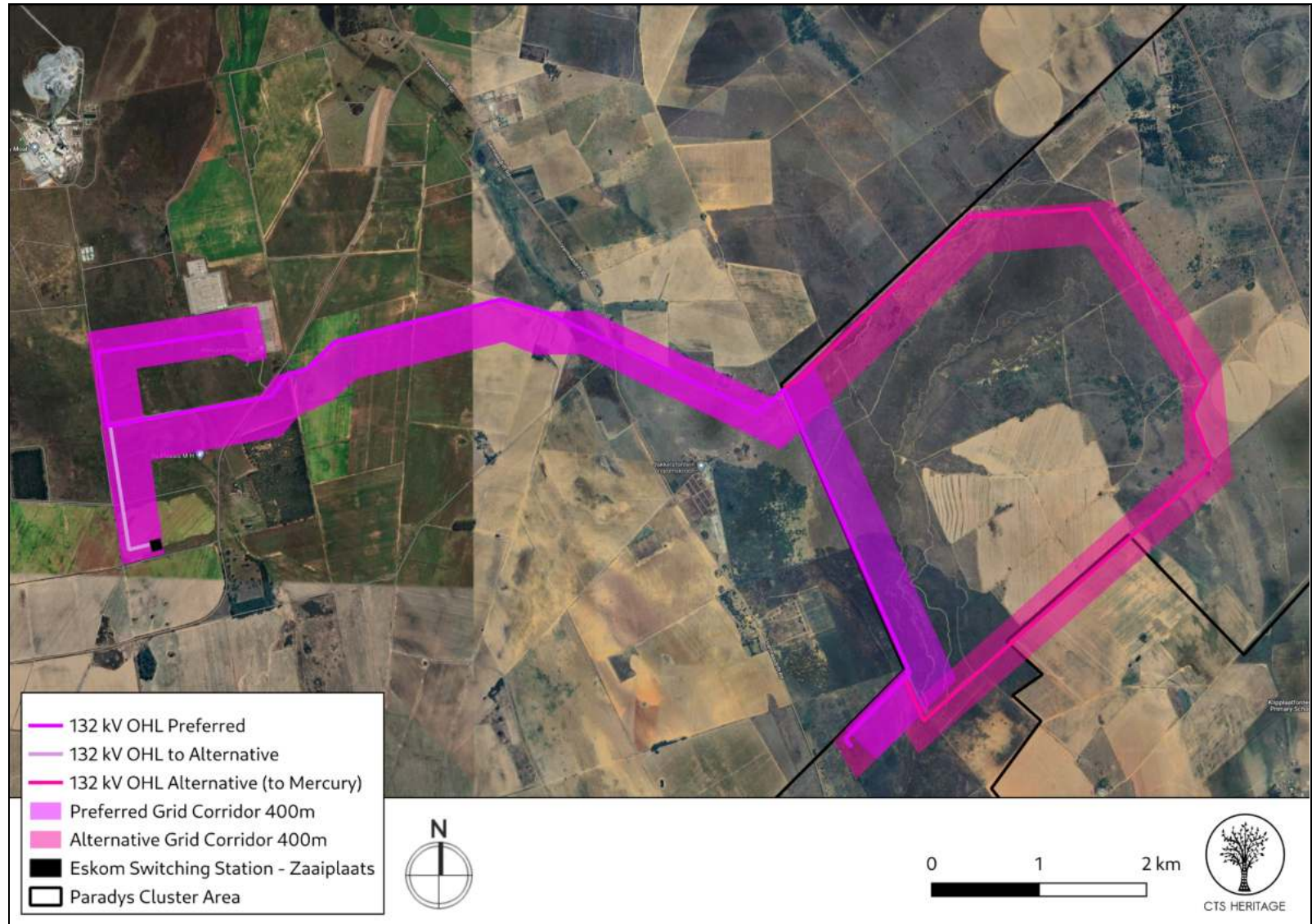
Figure 1.3: The proposed development layout of the Mooiwater Solar PV EGI
