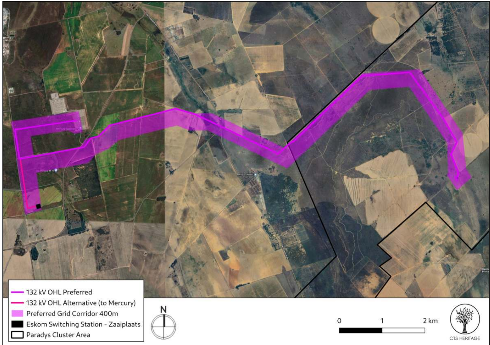
Figure 1.3: The proposed development layout of the Rudolph Solar PV EGI
