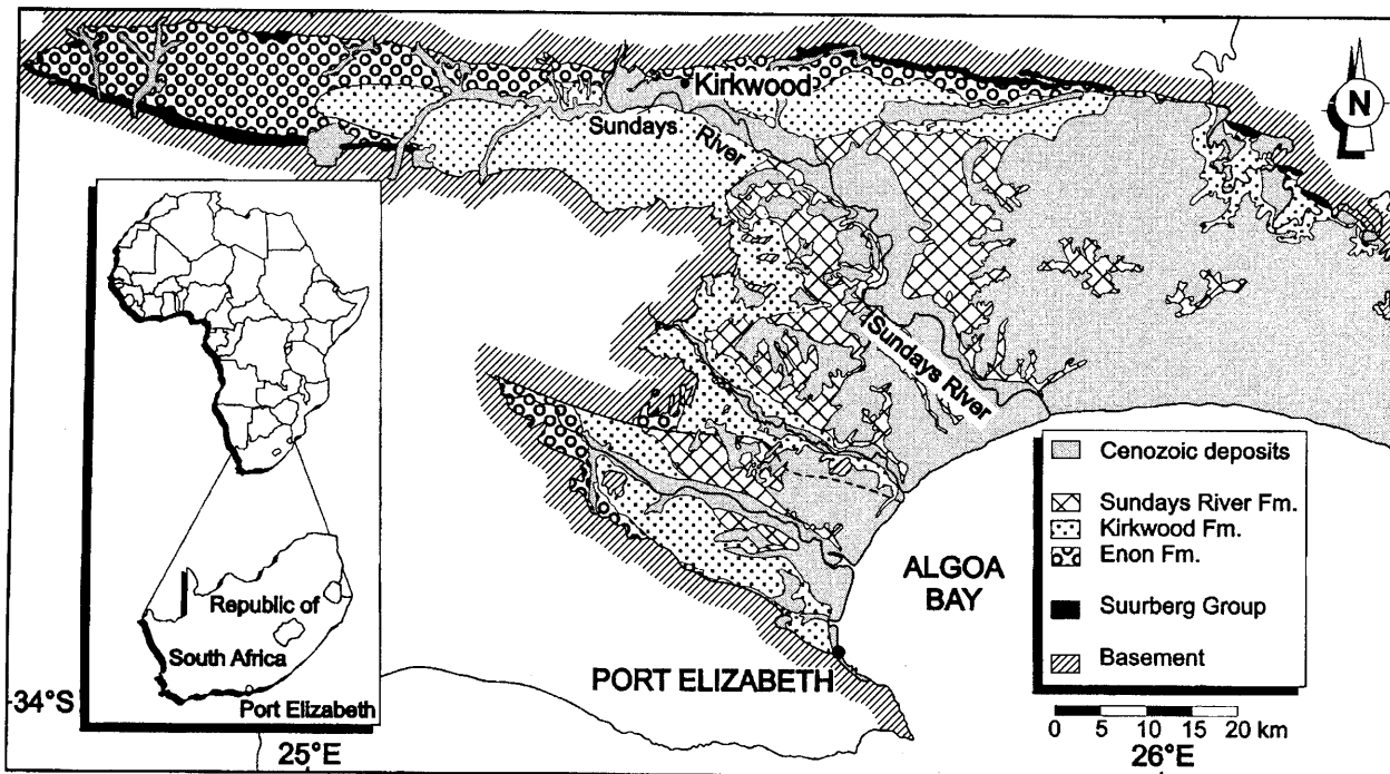
Fig. 5. Outcrop map of the main formations of the Mesozoic Uitenhage Group within the Algoa Basin (From Gomez et al. , 2006b). Note the extensive cover by Late Caenozoic sediments of the Algoa Group close to the coast.
