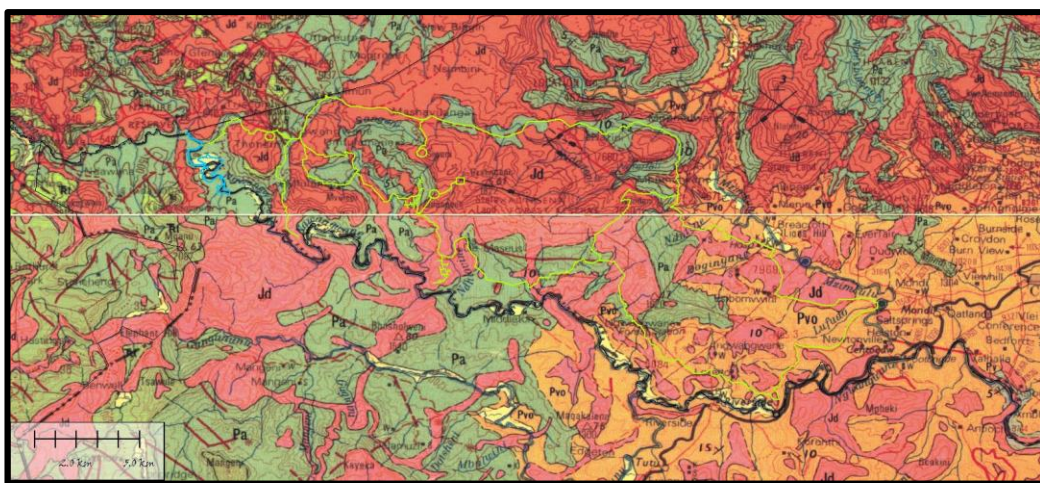
Figure 2 Geology underlying the study area includes the Volksrust Formation (Pvo) of the Ecca Group, the Adelaide Subgroup (Pa) of the Beaufort Group and Dolerite (Jd)
