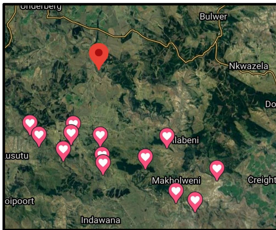
Figure 5 Points where specific recordings of fossils or unique geological features were observed as reported in Table 2
