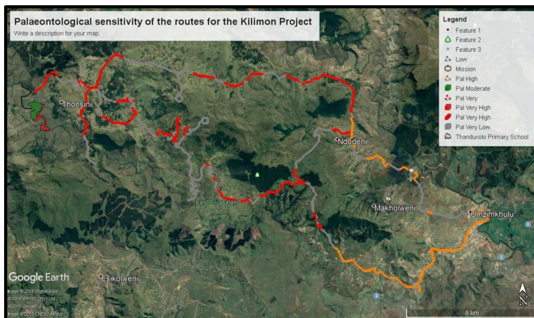
Figure 6 Palaeontological Sensitivity of the rocks underlying the Kilimon Project area. For colour codes see Table 1
