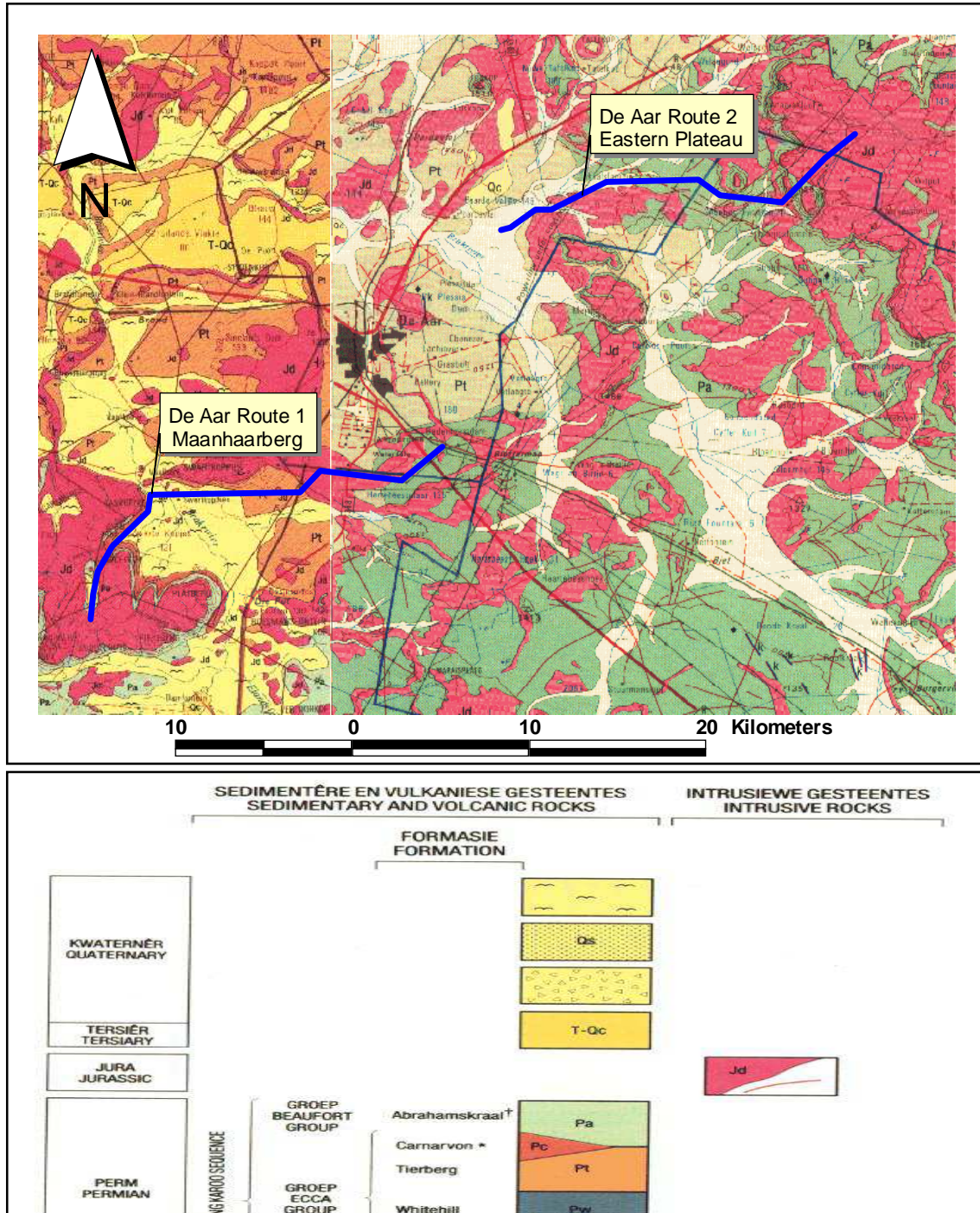
Figure 21 Geology of the study area at De Aar (Geo Maps 3022 Britstown and 3024 Colesberg)
