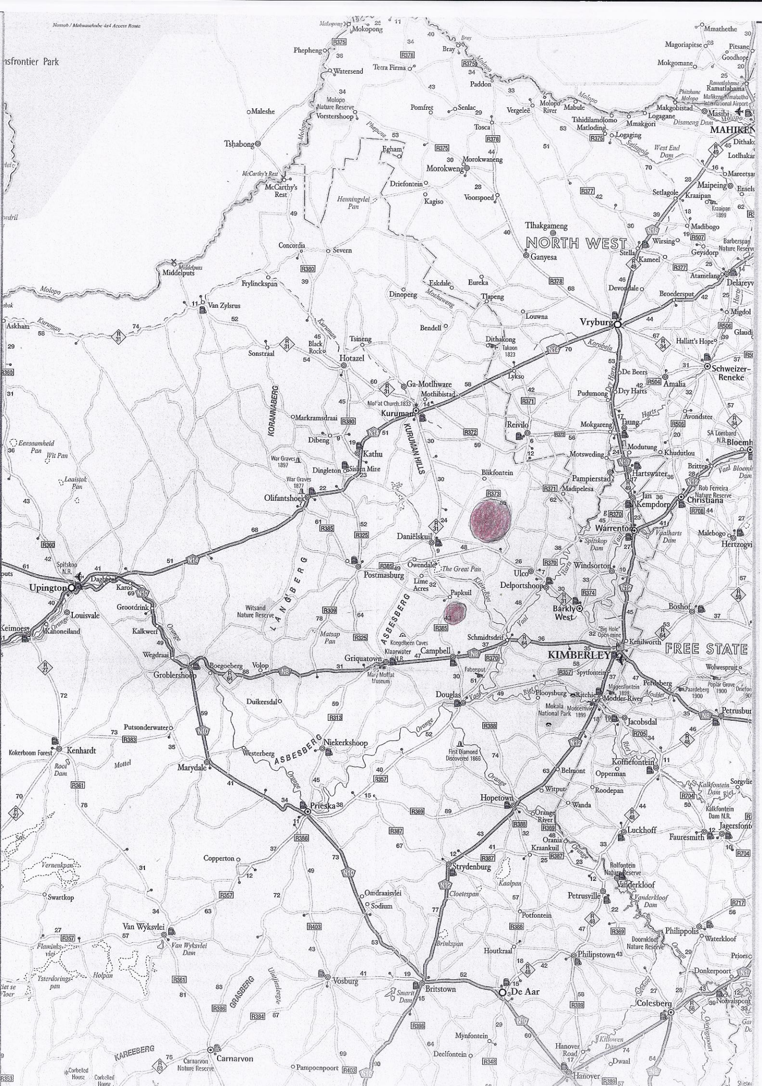
FIG 1. REGIONAL MAP SHOWING THE POSITION OF THE KIMBERLITE GLUSTERS NORTH OF CAMPBELL AND EAST OF DANIELSKUIL.
