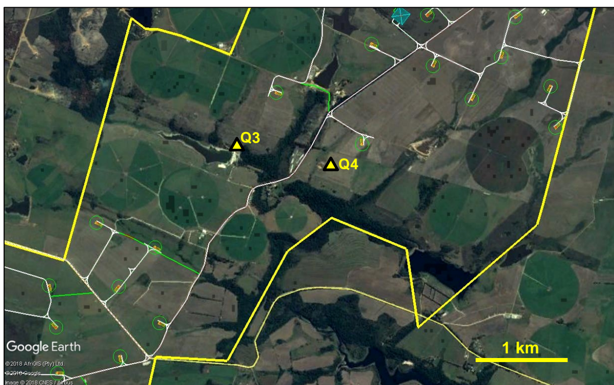
Figure 6. Google Earth© satellite image of the central part of the Impofu West Wind Farm project area showing the location of two sites of palaeontological / geoheritage interest near Rosenhof farmstead: Q3 quarry (important trace fossil assemblages within the Peninsula Formation) and Q4 quarry (ferricretised Nanaga Formation with ESA stone artefacts). These two sites will not be directly impacted by the proposed wind farm development, although located within the proposed wind farm boundary.
