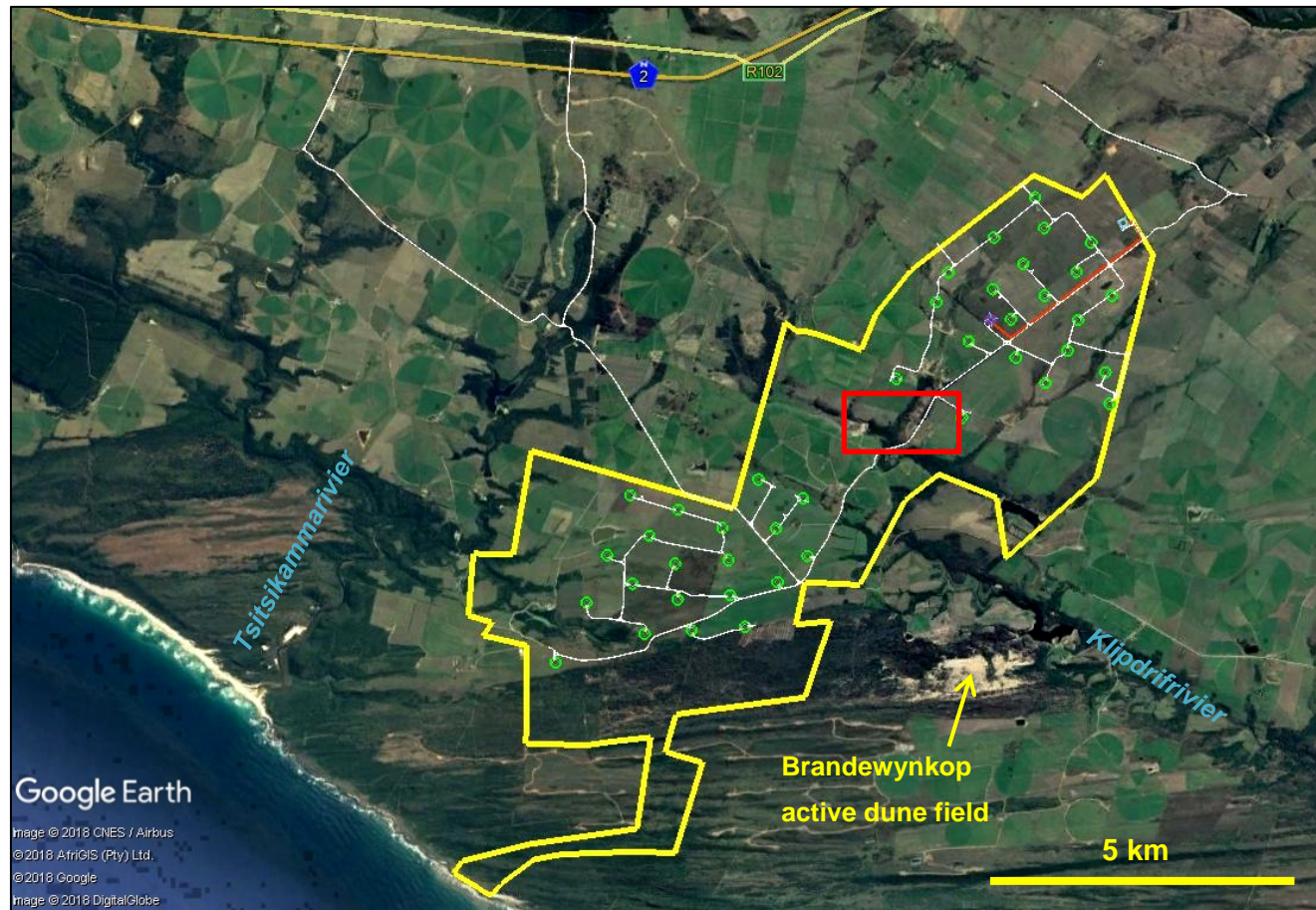
Figure 3. Google Earth© satellite image of the Impofu West Wind Farm study area (yellow polygon) spanning the coastal platform c. 25 km WSW of Humansdorp. The provisional development footprint is indicated, including wind turbine and standing area positions (green), access roads (white) and 132 kV line (red) from the on-site Impofu West Substation (small purple square). Two sites of geological / palaeontological conservation value lie within the small red rectangle (See Fig. 6 for more detail).
