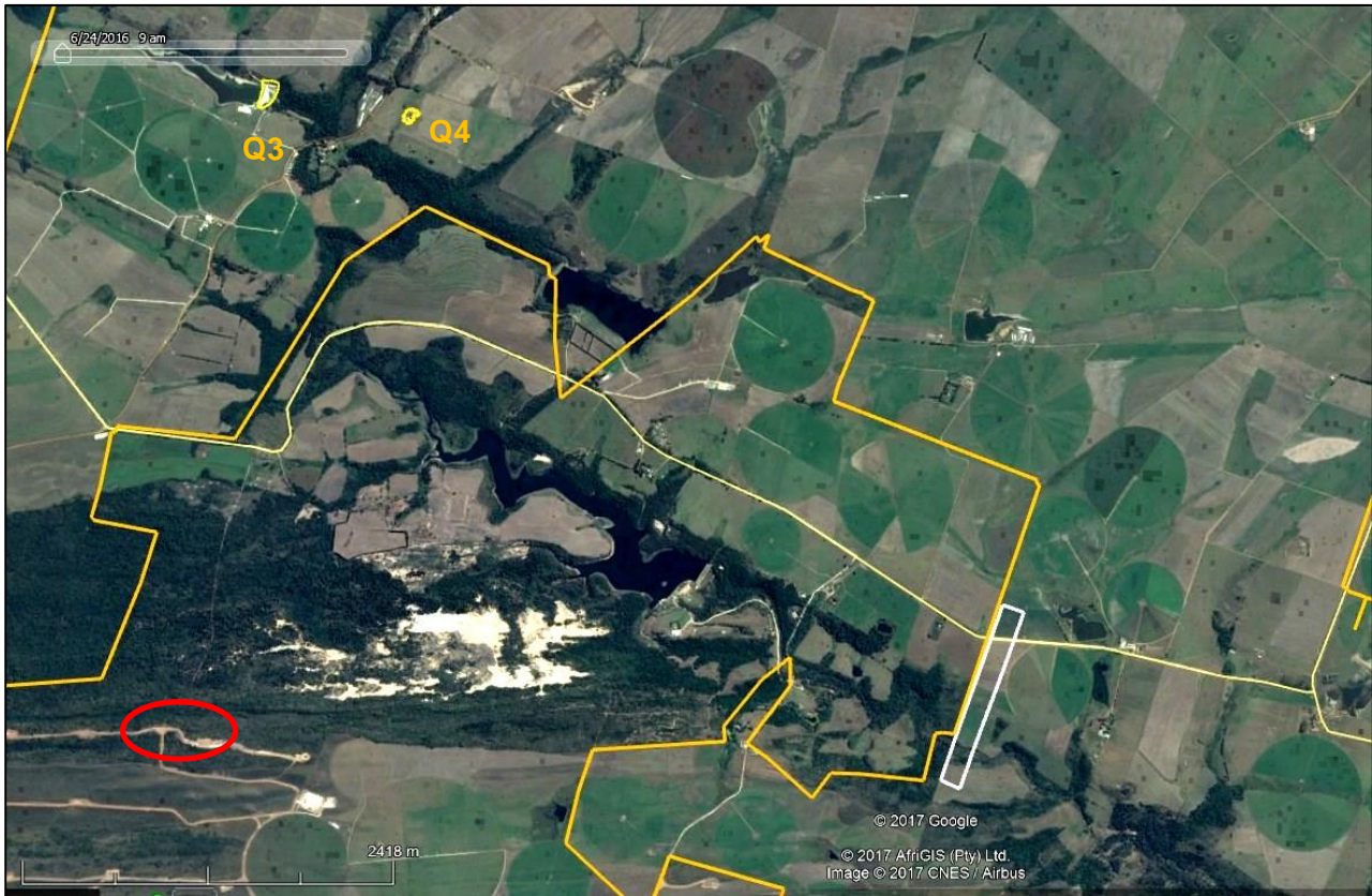
Figure 3. Satellite image showing the location of two quarry sites near Rosenhof farmstead. Q3 displays important trace fossils within the Peninsula Formation while Q4 is of geoheritage as well as archaeological interest. Both sites lie within the Impofu West Wind Farm study area. An important hyaena den accumulation of mammal bones and coprolites has been recorded in the area encircled in red to the southwest of the Brandewynkop dunefield (Nilssen & Smith 2015). New road and / or powerline developments across the valley of the Klipdrifrivier within the elongated white rectangle are of low palaeontological heritage significance.
