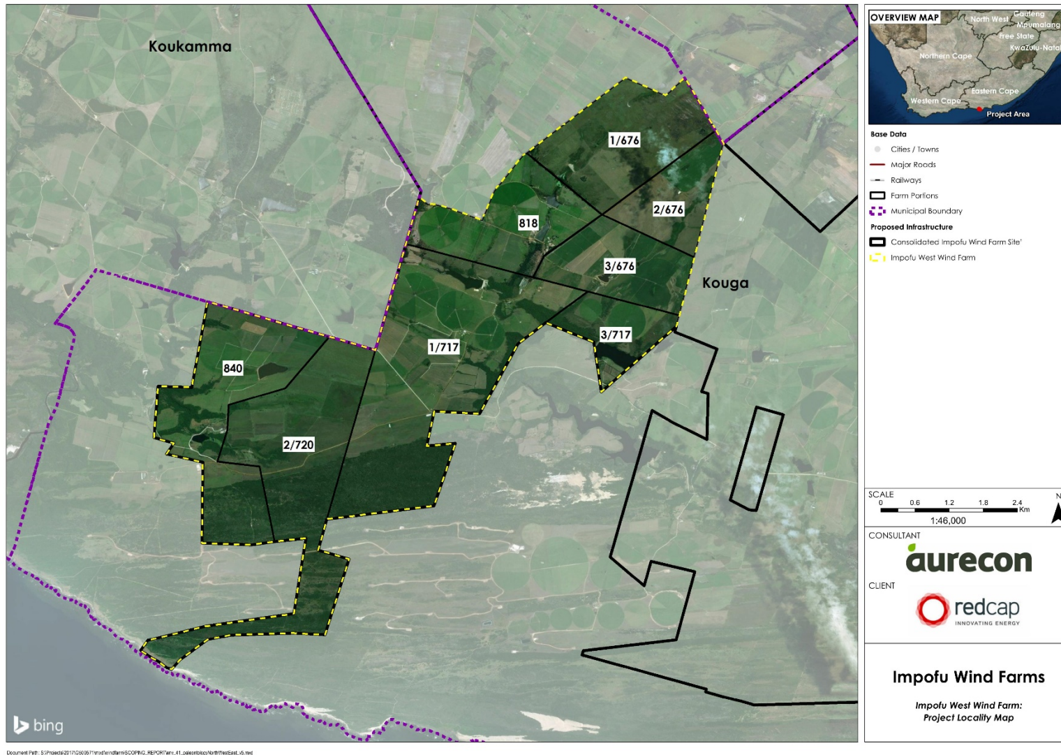
Figure 2: Map showing the location of the land parcels concerned in the proposed Impofu West Wind Farm located c. 25 km WSW of Humansdorp, Sarah Bartaan District Municipality, Eastern Cape (Image provided by Aurecon South Africa (Pty) Ltd).
