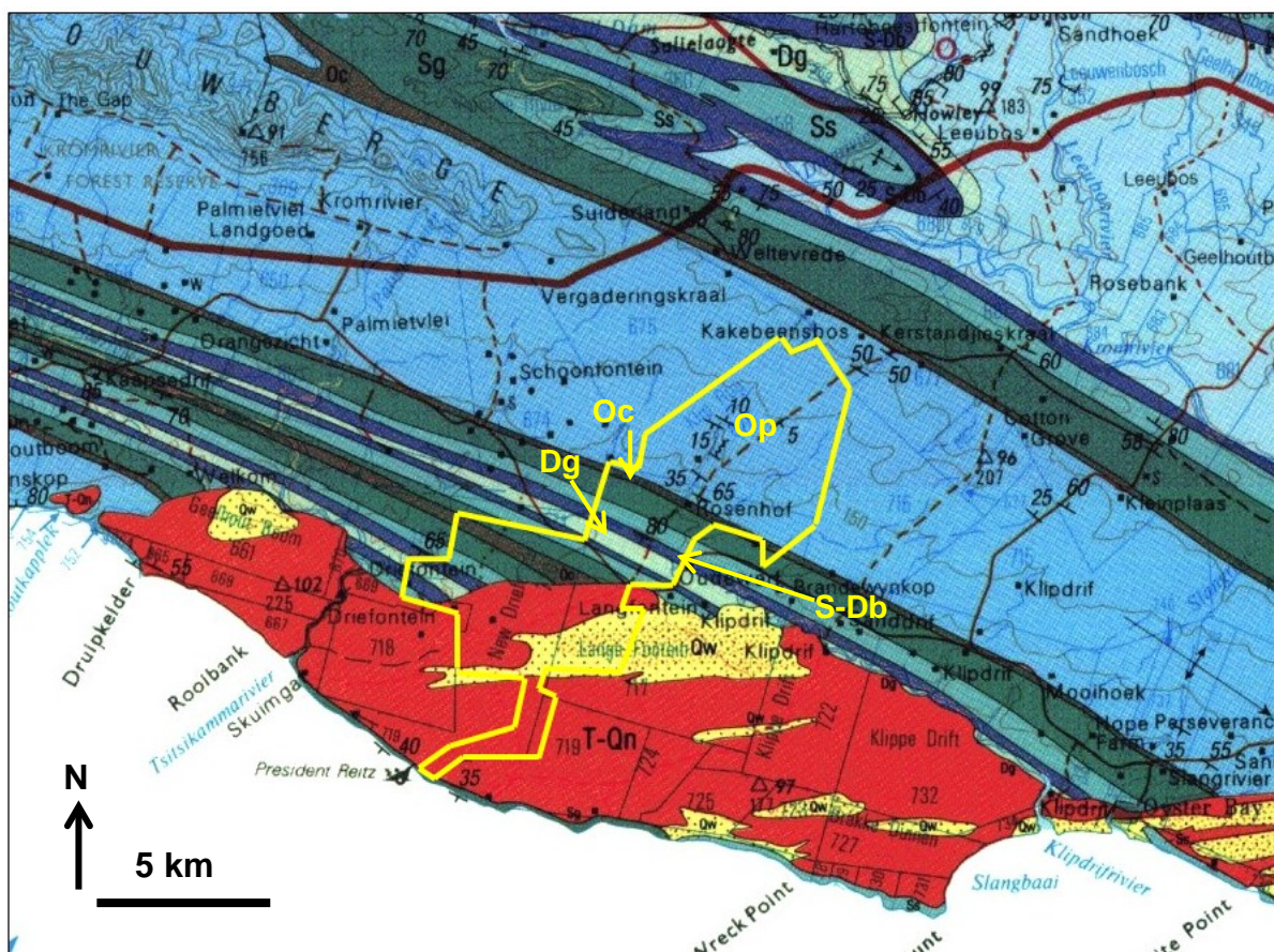
Figure 4. Extract from 1: 250 000 geology sheet 3324 Port Elizabeth (Council for Geoscience, Pretoria) showing approximate outline of the Impofu West Wind Farm study area near Humansdorp (yellow polygon). The main geological units represented within the study area include the following formations (Palaeontologically more sensitive marine units indicated in red below). Please note that geological mapping at 1: 250 000 scale in this region is often schematic due to very poor levels of bedrock exposure.
