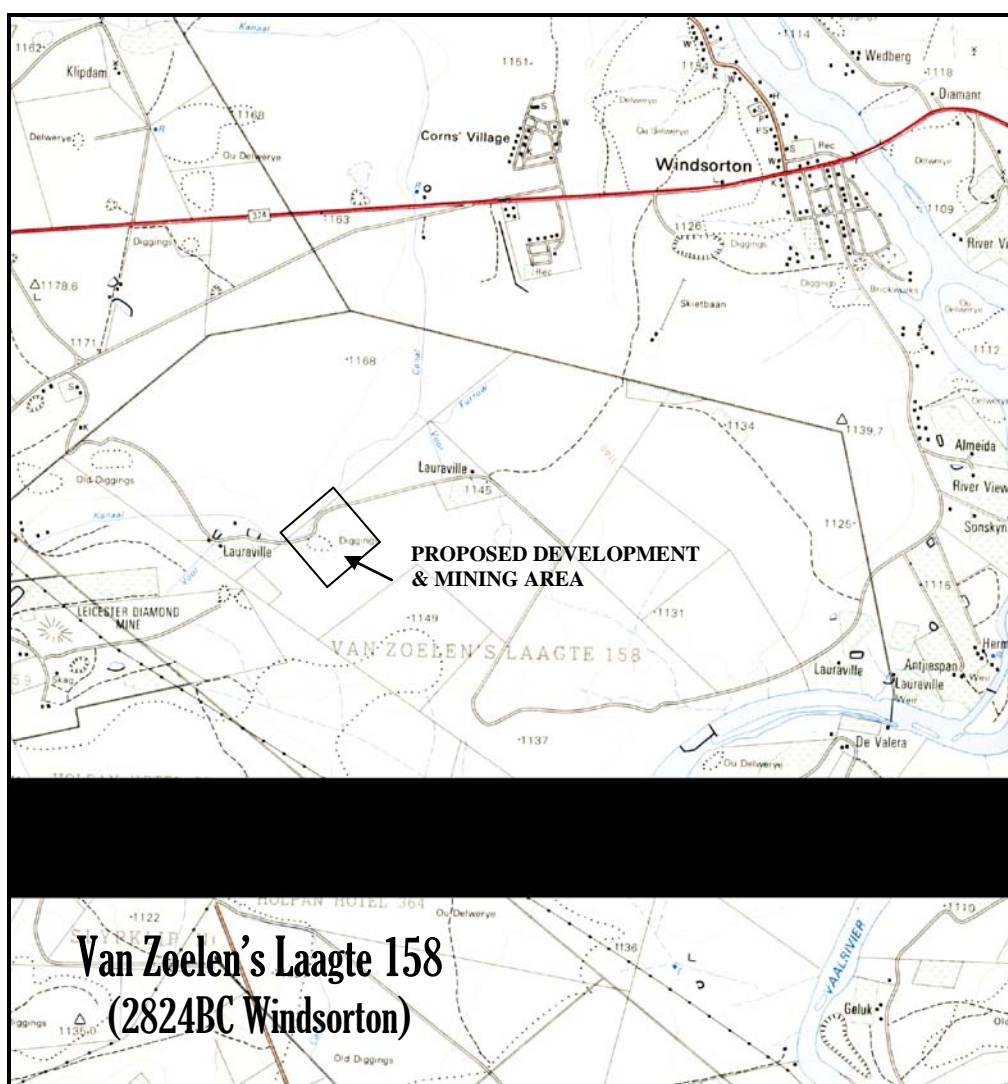
MAP 1: Extract of the 1:50,000 2824BC Windsorton map indicating the position of the proposed Van Zoelen's Laagte 158 development.
