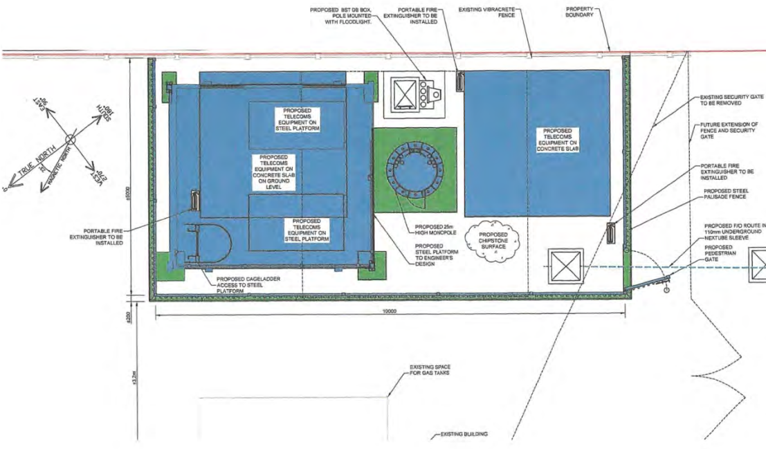
Figure 3. Layout (above) and plan of the proposed development (below).
