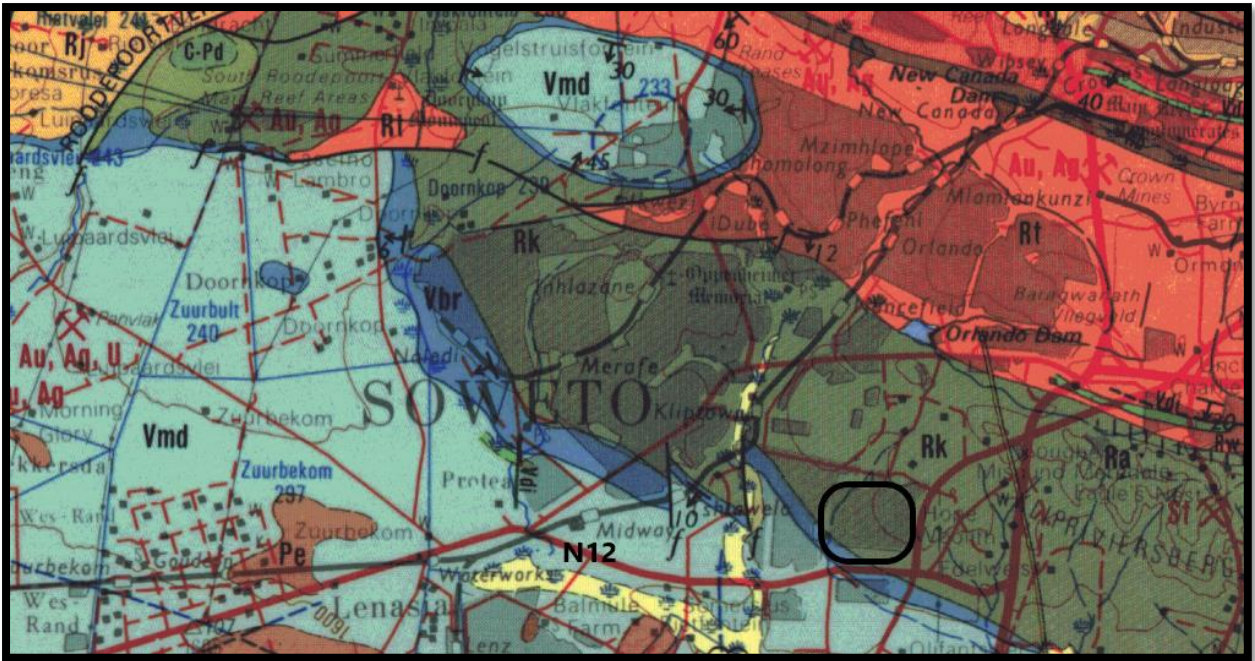
Figure 3: Excerpt of 1:250 000 Geological Map 2626 Wes Rand (Keyser 1986) (1h).
