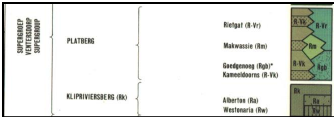
Figure 4: Lithostratigraphy (Keyser 1986).
