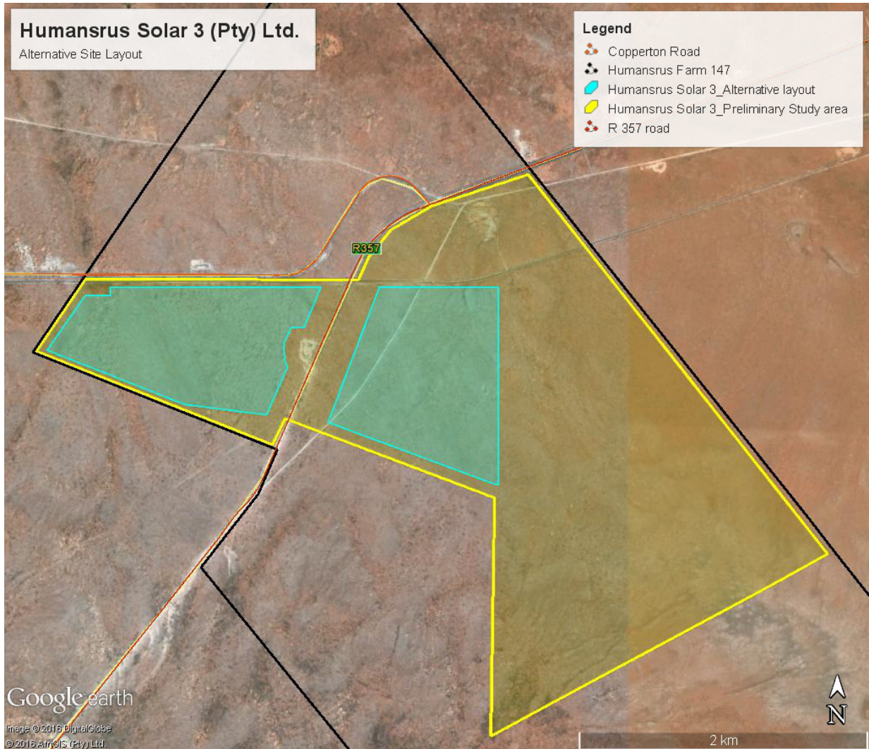
Figure 4: Proposed Alternative 2 (Solek, 2015)
