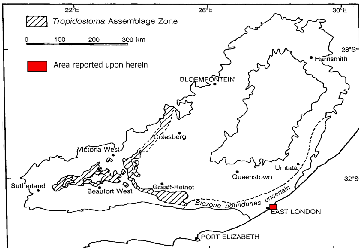
Figure 5: The distribution of the Tropidostoma Assemblage Zone in South Africa. The Tropidostoma Assemblage Zone is one of the vertebrate biostratigraphic zones that may be present in the rocks underlying the project area. It is evident from the diagram that the status of the vertebrate-based biostratigraphy in the rocks underlying the project area is uncertain (Modified from Smith and Keyser, 1995).
