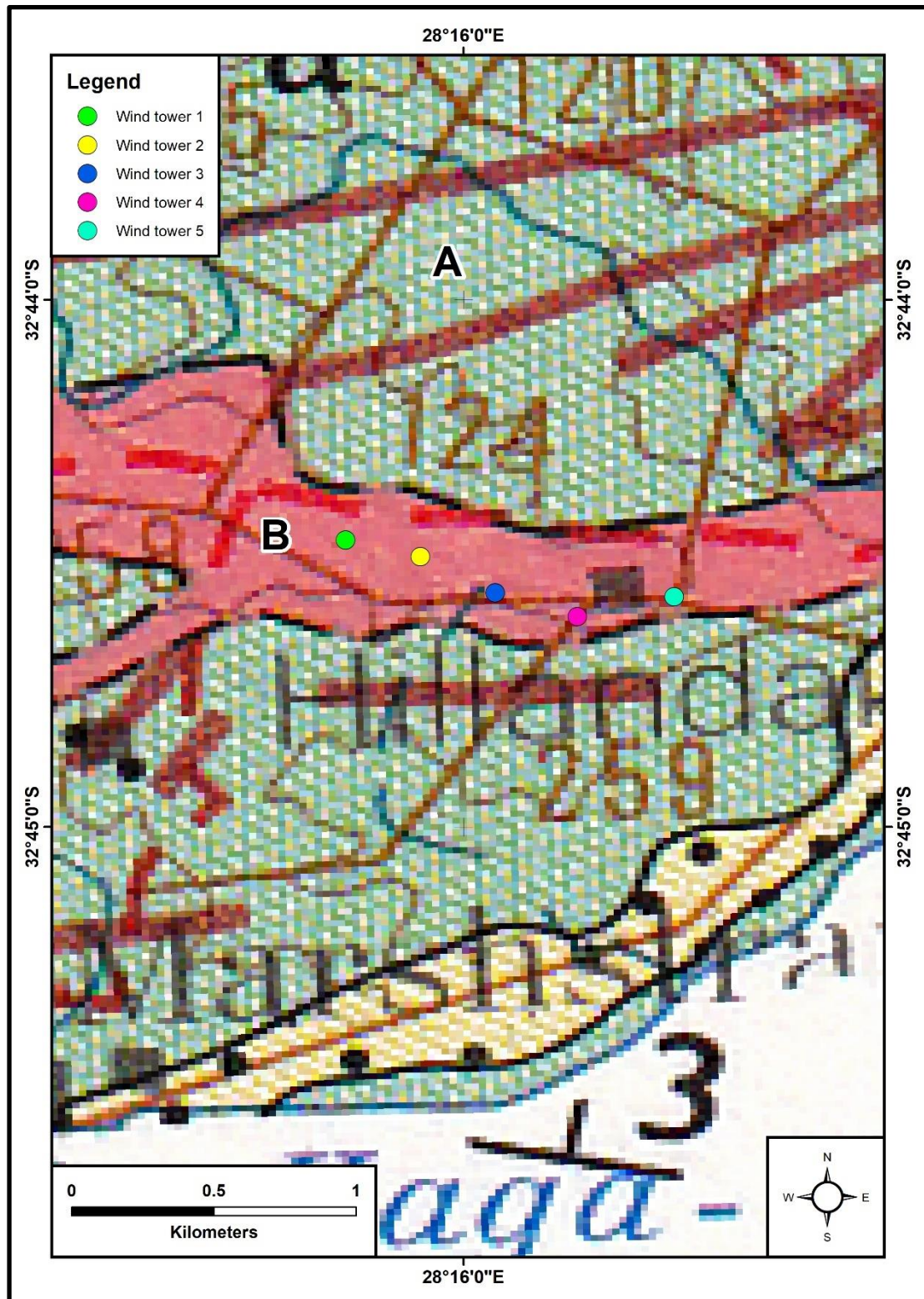
Figure 4: Geological map of the area underlying the proposed project infrastructure and the surrounding environs. The stratigraphic unit marked "A" is the Adelaide Subgroup while the unit marked "B" is the Karoo Dolerite Suite (Modified from Geological Survey of South Africa, 1979).
