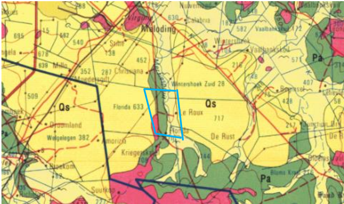
Figure 4: Geological map of the area around the Florida 1 & 2 Solar Parks within the blue outline. Abbreviations of the rock types are explained in Table 2. Map enlarged from the Geological Survey 1: 250 000 map 2826 Winburg.
