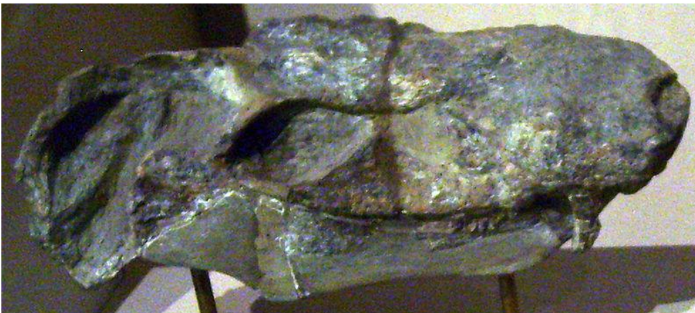
Figure 11 : Pristerognathus skull
