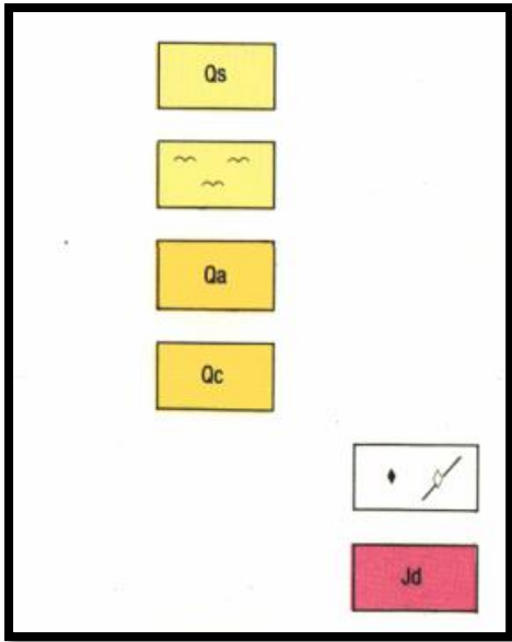
Figure 5: Lithology (Kimberley 2824).
