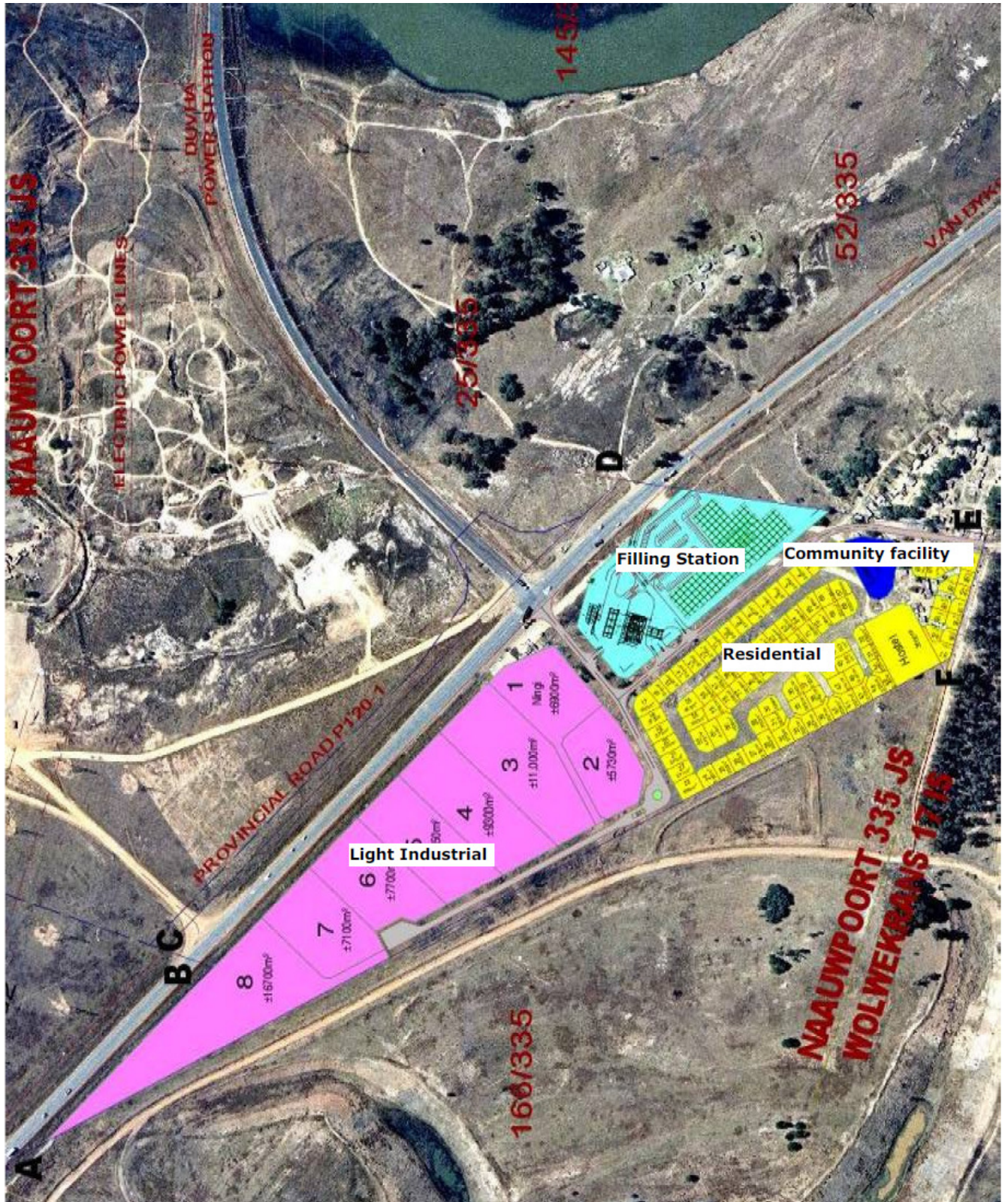
Figure 4 Site development plan.
