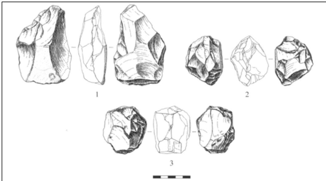
Figure 6. (1) handaxe on flake; (2) thick discoidal core; (3) polyhedral core (Pollarolo, Kuman, Bruxelles, 2010)
