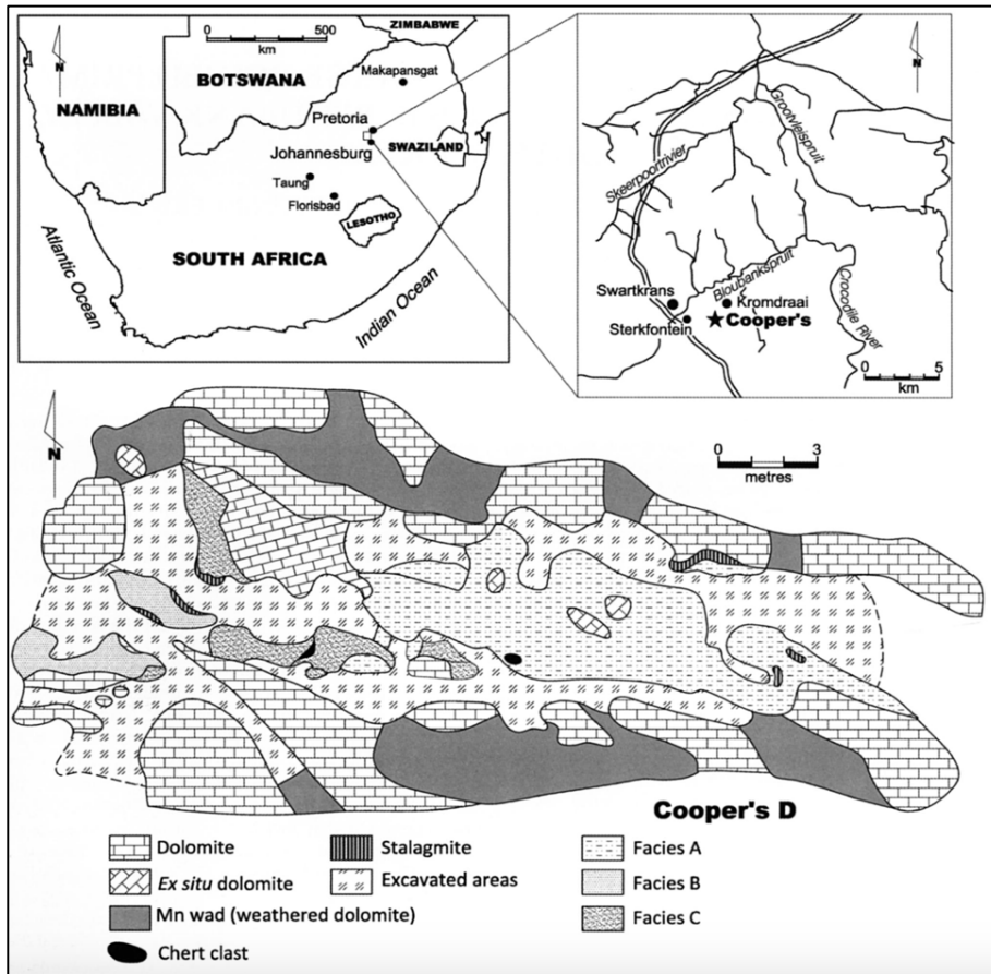
Figure 8. Geology and deposits at Cooper's Cave (Pollarolo, Susino, Kuman, 2010)
