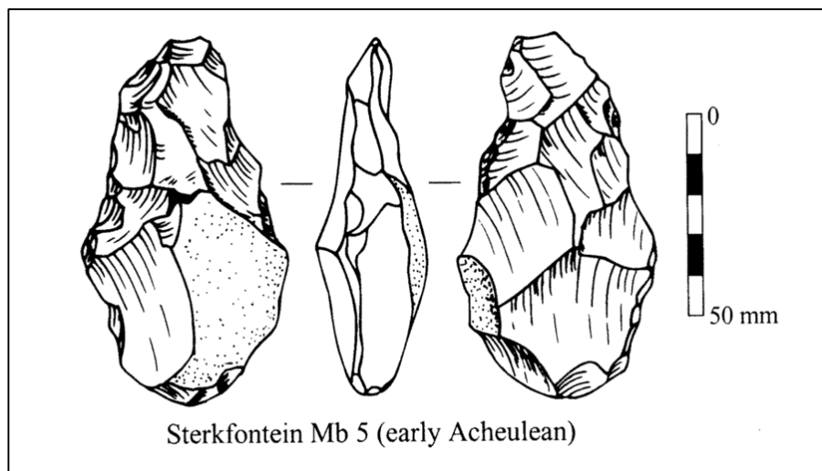
Figure 7. Azheulean handaxes from Sterkfontein (Val, Taru, Steininger, 2014)
