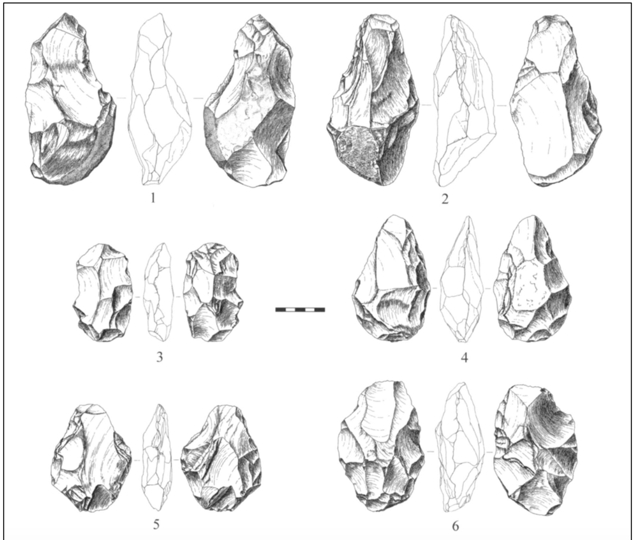
Figure 10. Handaxes from Coopers Cave (Pollaro, Susino, Kuman, 2010)
