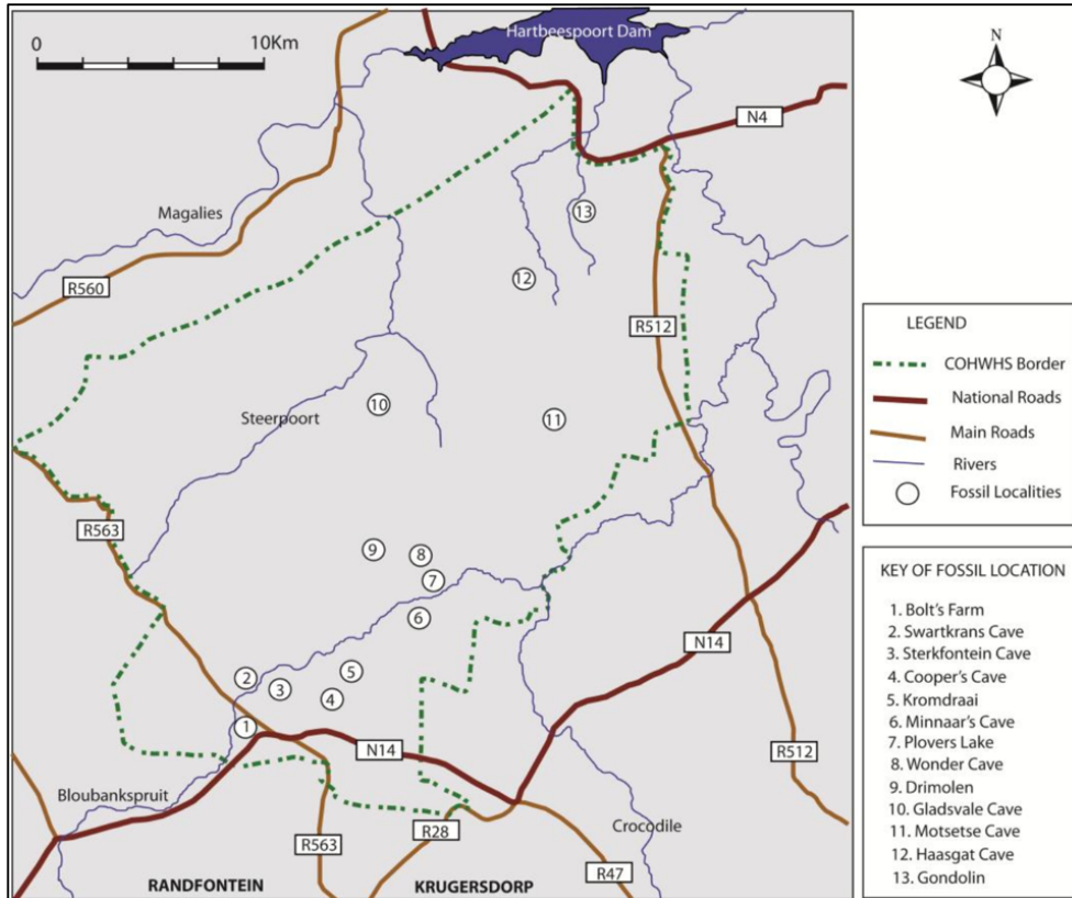
Figure 5. Important fossil sites at COH
