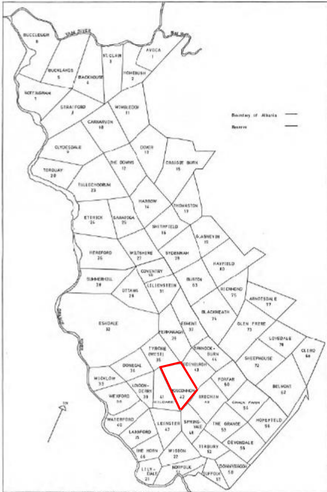
Figure 6. The Albania Settlement farms (Kurz 1988).
