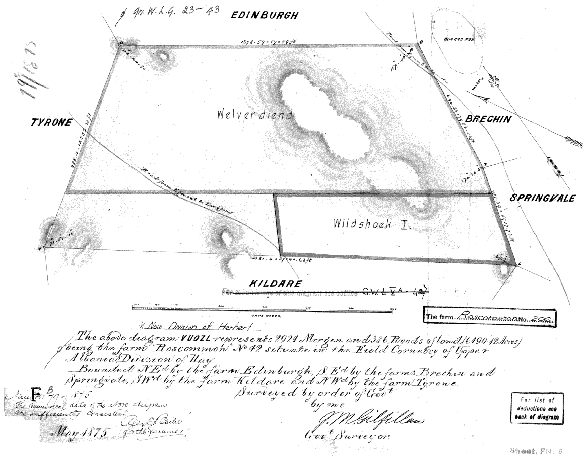
Figure 5. Copy of the May 1875 survey diagram indicating Roscommon, Field Cornetcy Upper Albania, Division of Hay (subsequently assigned to Herbert).
