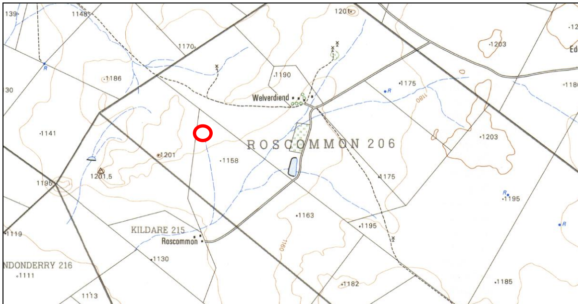
Figure 3. Portion of 1:50 000 sheet 2924AC showing Roscommon 206 and the location of the drill site.
