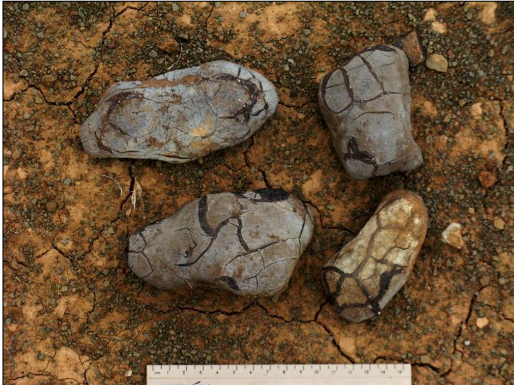
Figure 13: Ovoid grey calcrete nodules showing septarian cracking, surface gravels in bare patch on Kwanselaarshoek 40 (Loc. 010) (Scale in cm).
