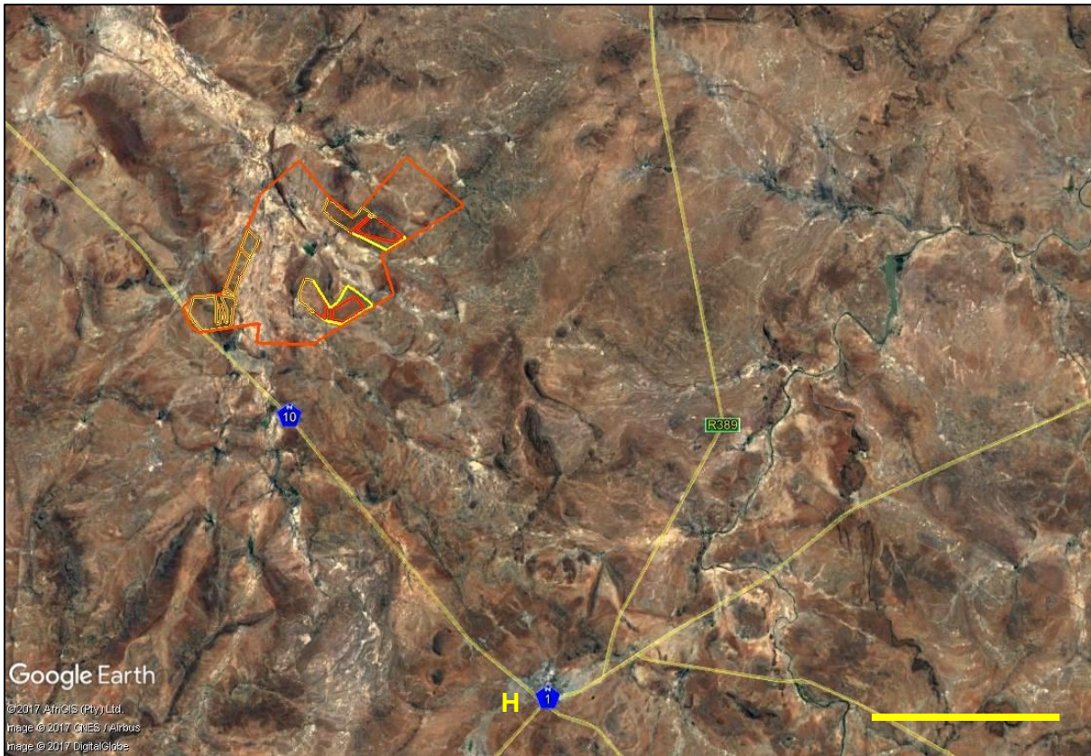
Figure 1: Google Earth satellite image showing the location of the proposed Soventix solar PV plant some 30 km northwest of Hanover (H), Northern Cape (Scale bar = 10 km.). Three interconnected solar plant sites (1,2,3) make up the integrated PV project (See Fig. 2).
