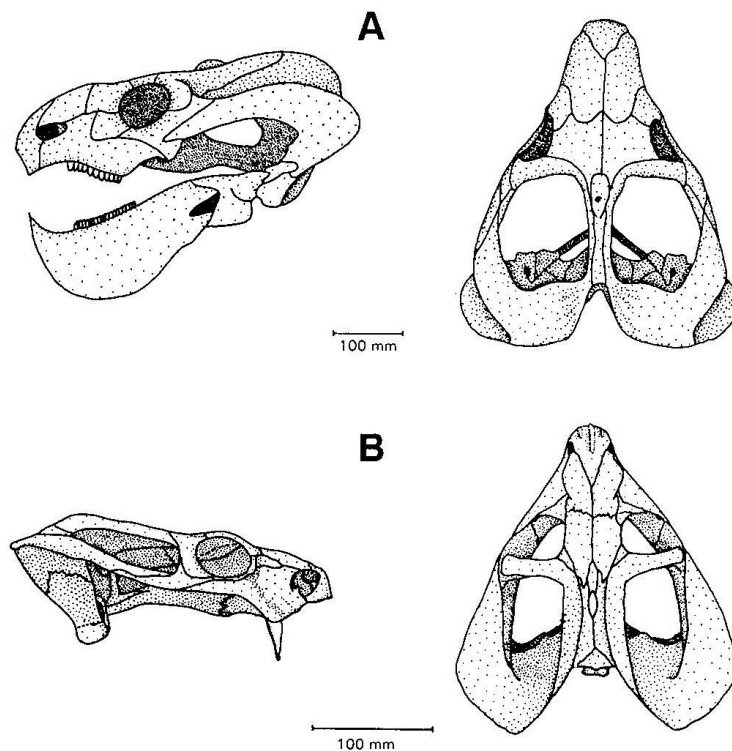
Figure 23: Skulls of two important medium-sized dicynodont therapsids that characterise the Tropidostoma Assemblage Zone: A – Endothiodon ; B – Tropidostoma (From Smith & Keyser 1995).
