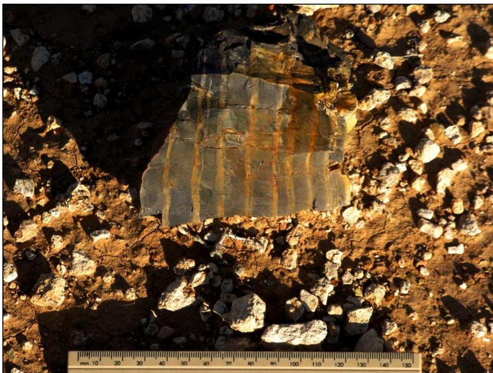
Figure 29. Larger angular block of silicified wood showing clear seasonal growth-banding from calcretised older alluvium on Rietfontain 39 (Loc. 020) (Scale in cm and mm).
