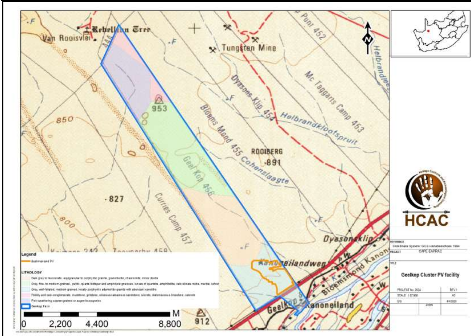
Figure 5. Lithology of the study area.
