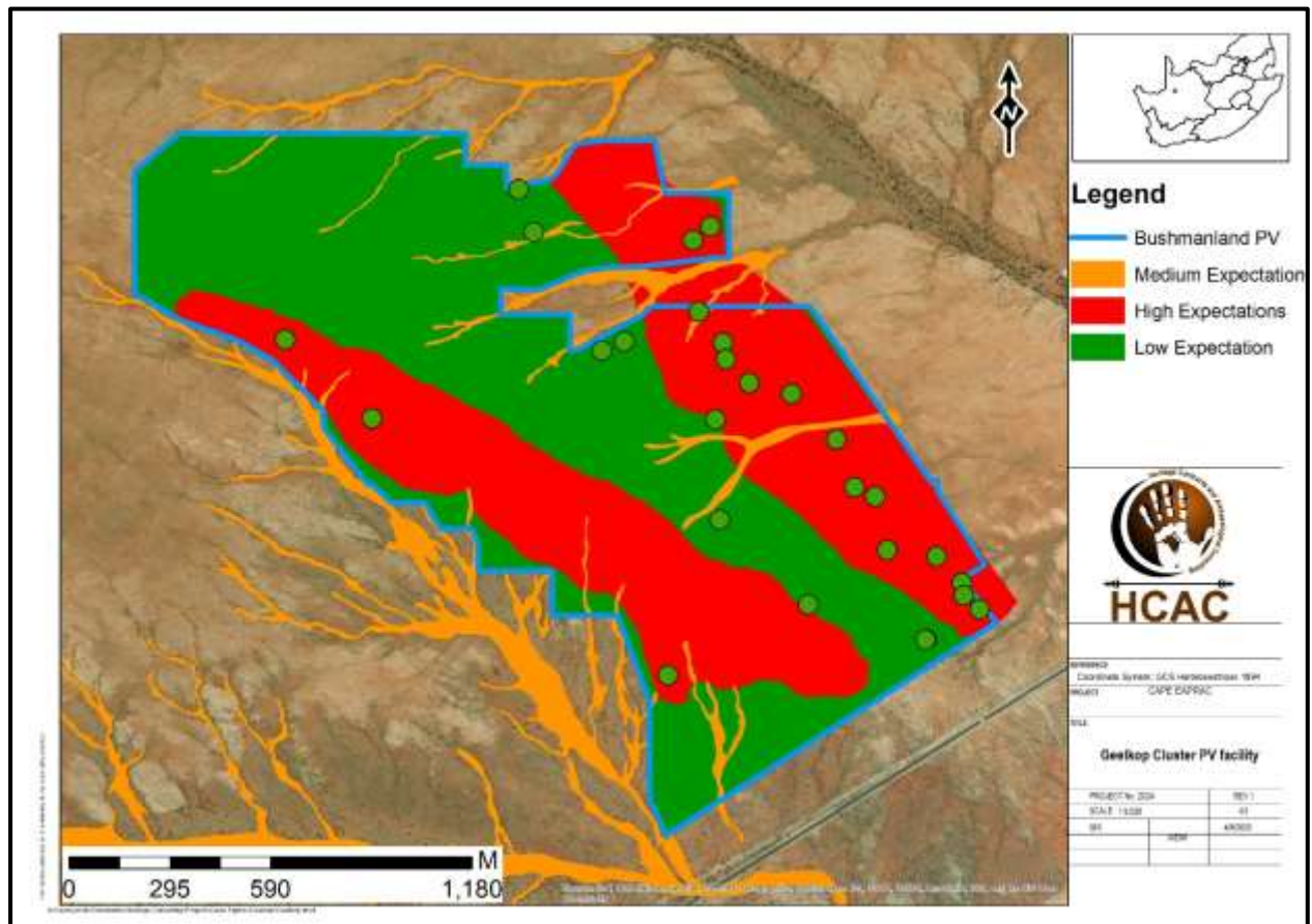
Figure 17. Predictive model vs sites
