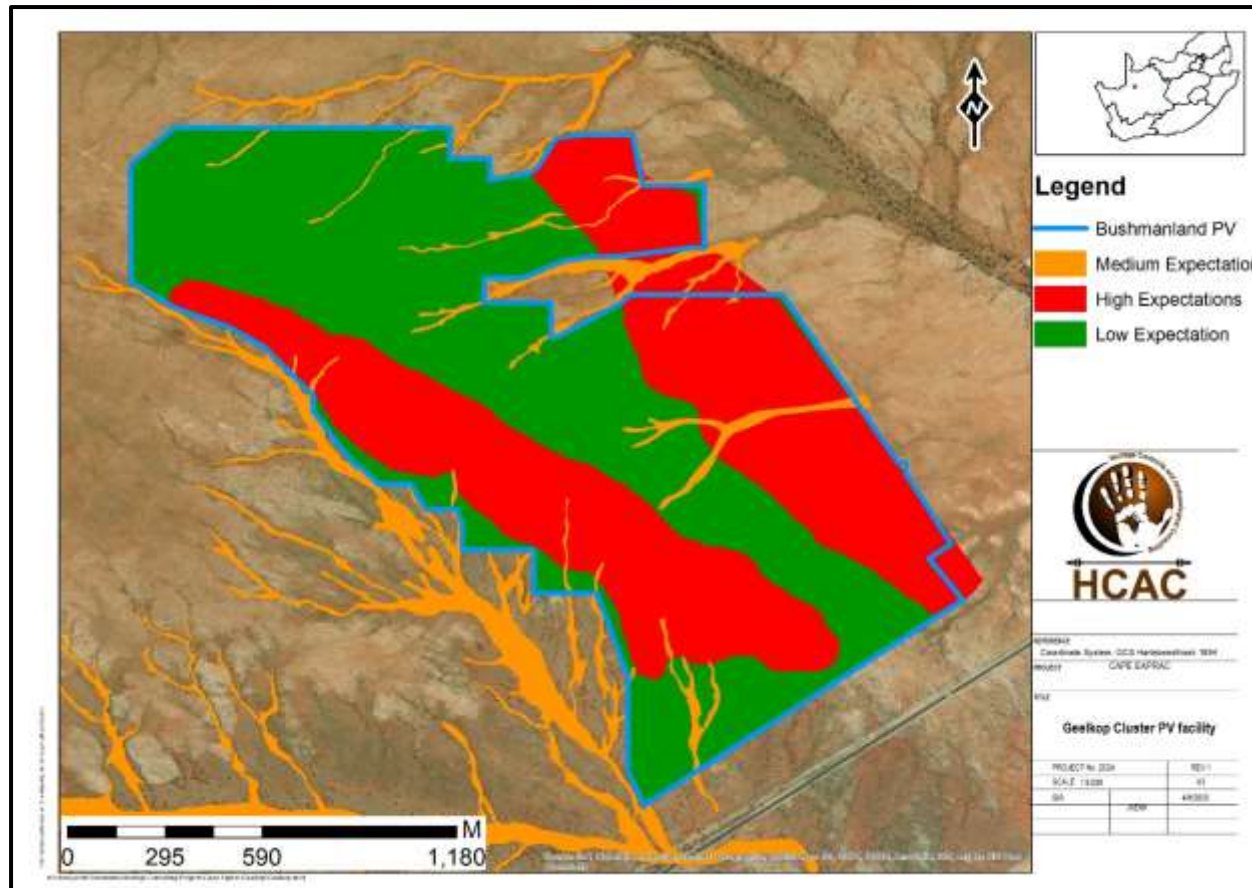
Figure 14. Graphic representation of the Predictive Model.
