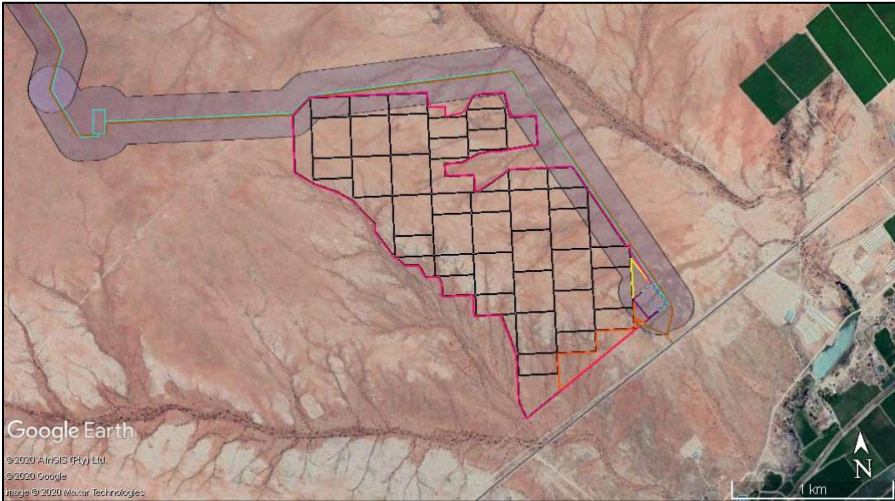
Figure 3. Satellite image indicating the proposed PV layout (Google Earth 2019).
