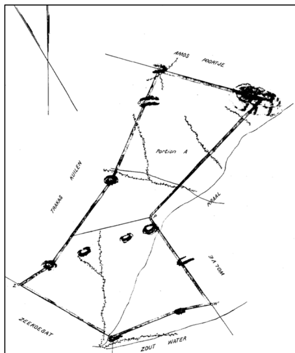
Figure 30: SG Diagram for Witpoortje 1872.
