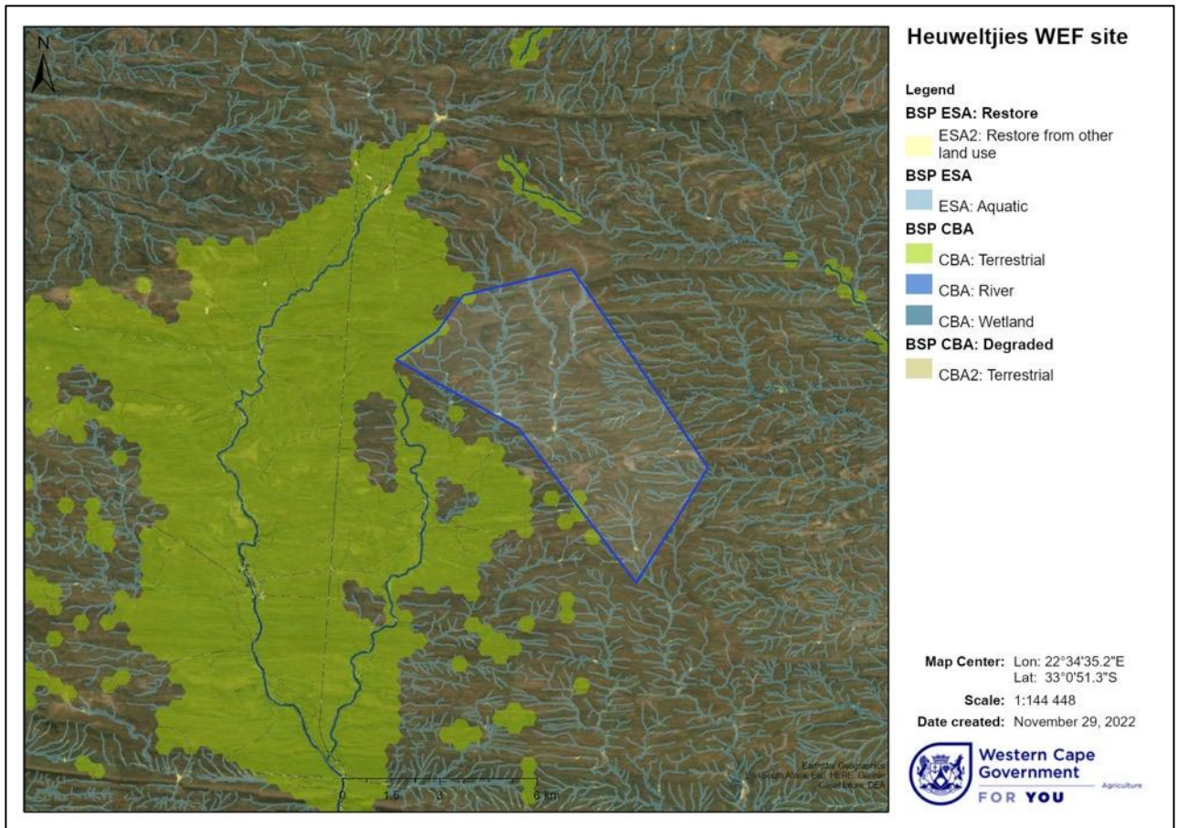
Figure 28: Critical Biodiversity Areas and Ecological Support Areas map for Heuweltjies landscape with proposed WEF site overlay.
