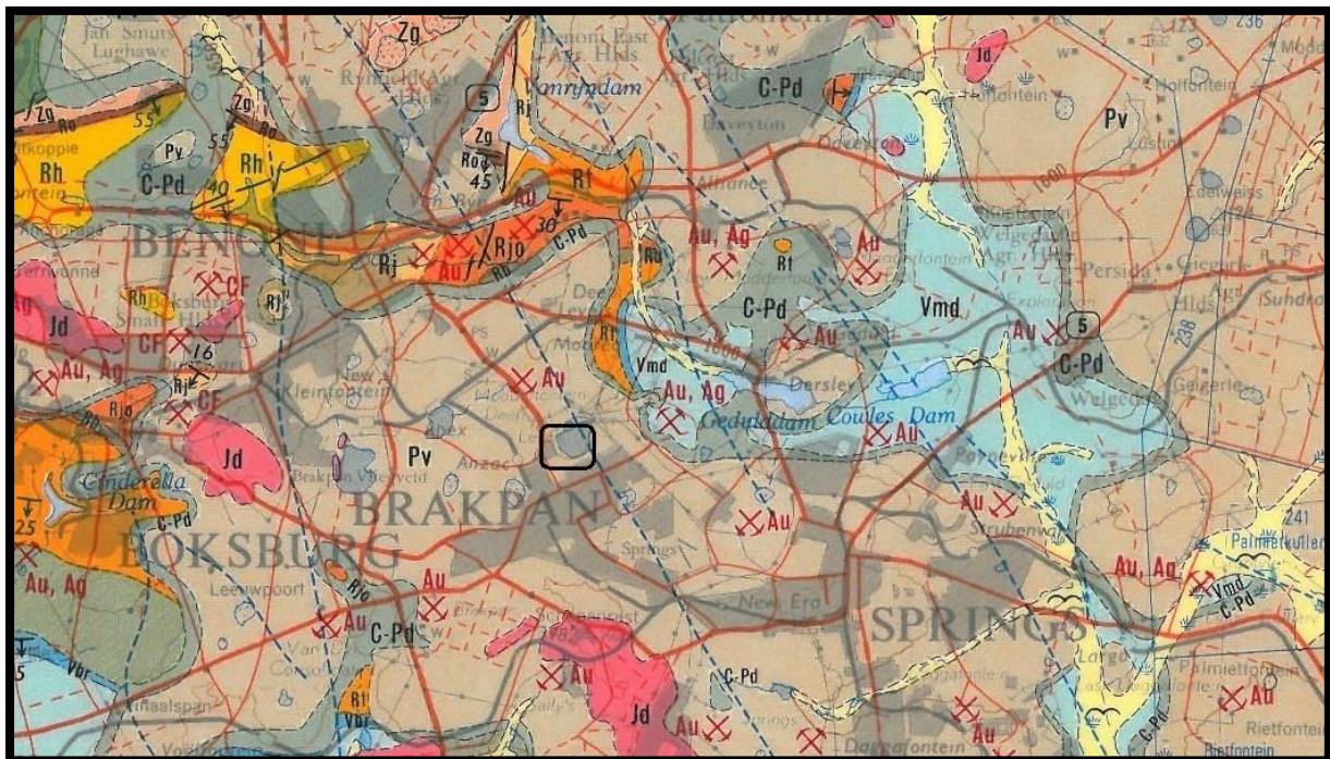
Figure 3: Excerpt of 1:250 000 Geological Map 2628 East Rand (Keyser et al. 1986).
