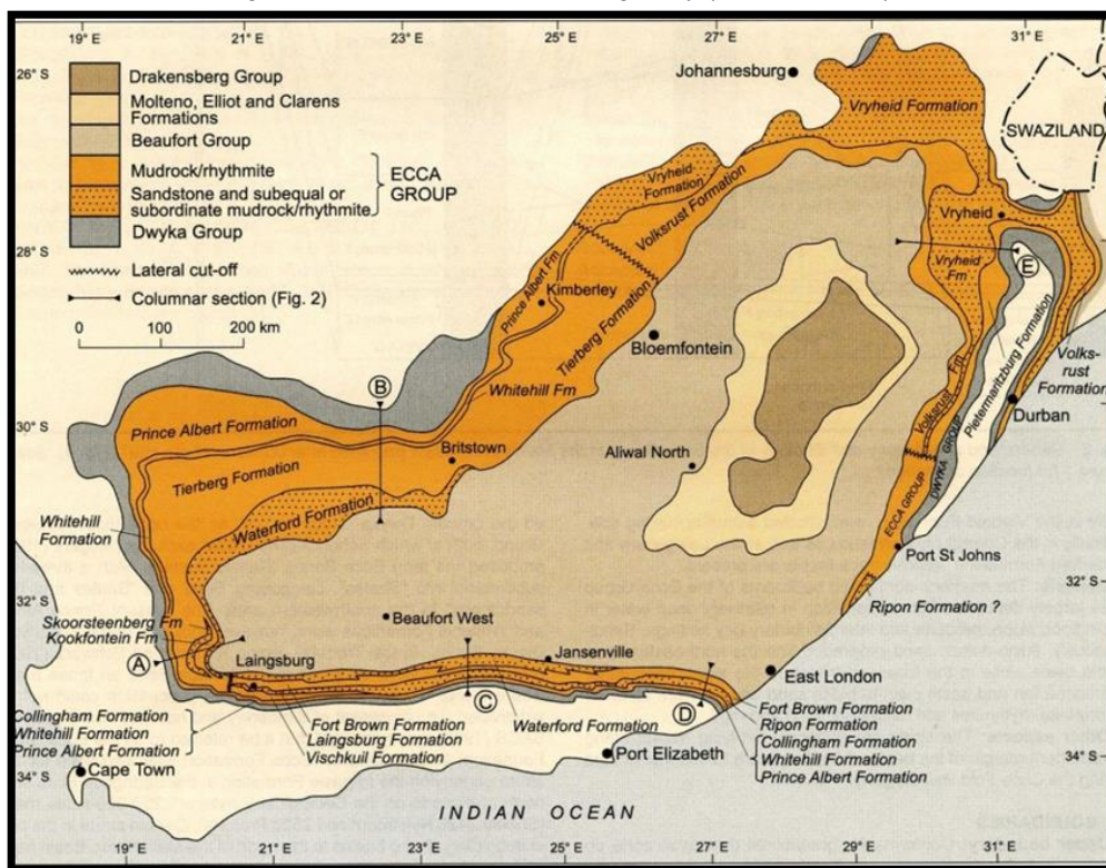
Map 1: Karoo Supergroup distribution and lithostratigraphy (Johnson 2009).
