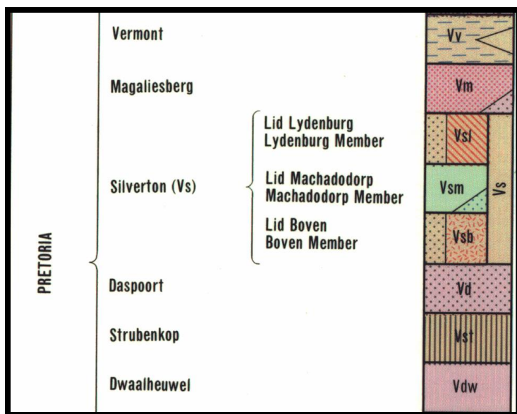
Figure 4: Lithostratigraphy (2430 Pilgrims Rest).
